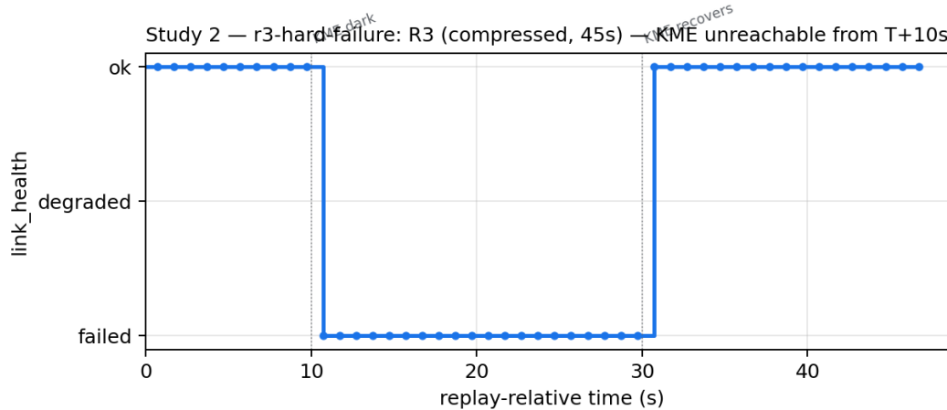
Figure 6. Study 2 — R3 hard-failure timeline. The KME is forced unreachable at T+10s and recovered at T+30s; the collector captures the Ok → Failed → Ok cycle on the next poll (observation latency ≈ 0.7s on the configured 1s interval).
