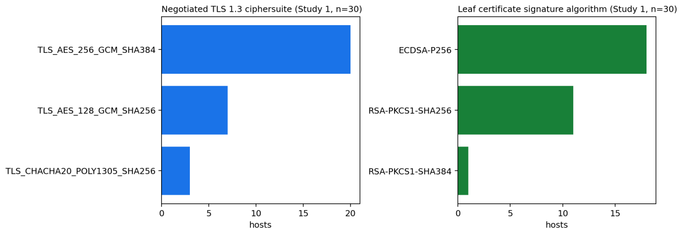
Figure 4. Study 1 — classical-probe baseline (n=30): negotiated TLS 1.3 ciphersuite (left) and leaf certificate signature algorithm (right). All 30 hosts negotiate TLS 1.3.
