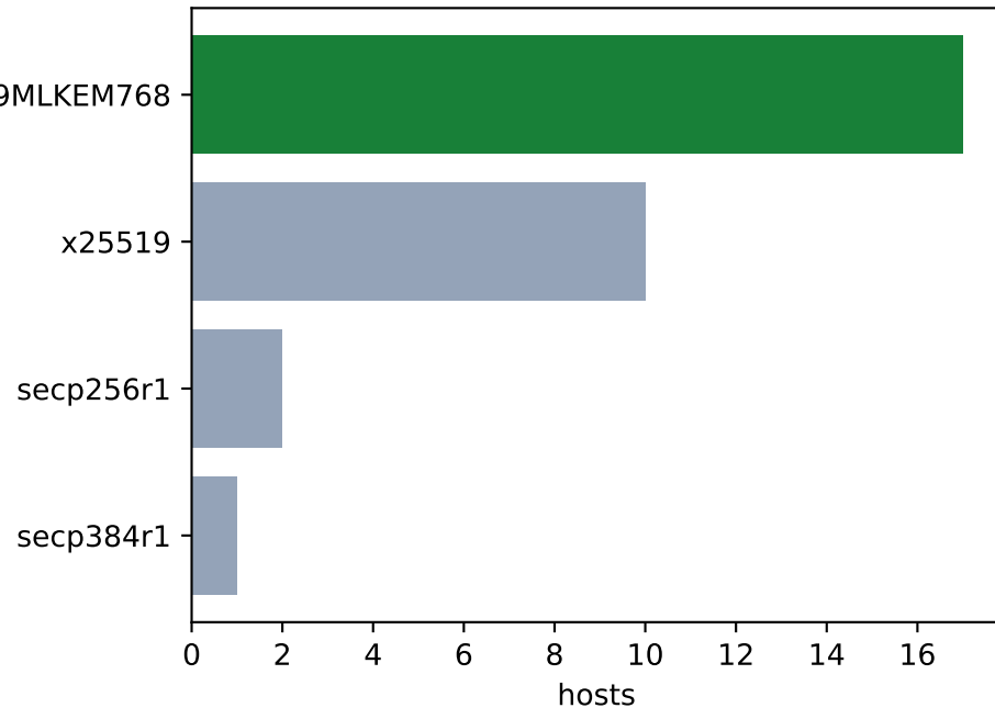
Negotiated key-exchange group (PQ-capable client)
