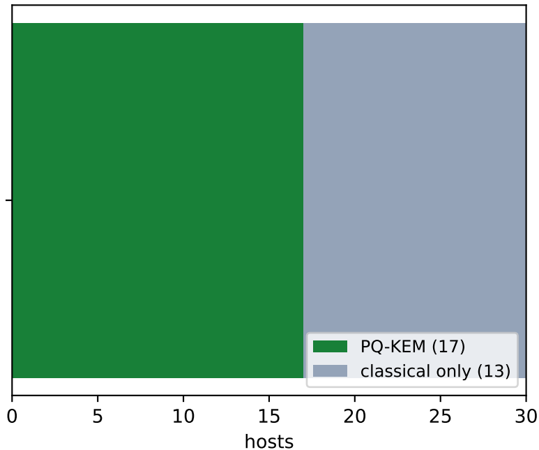
PQ-KEM negotiation when client advertises X25519MLKEM768 (rustls + rustls-post-quantum; 17/30 = 57%)
