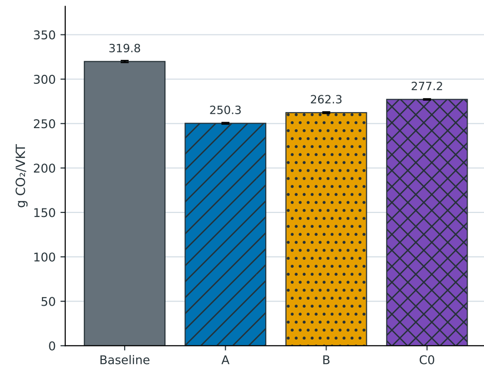
Tailpipe CO 2 intensity
