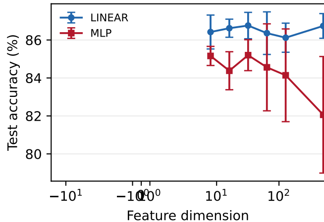
Fashion-MNIST
