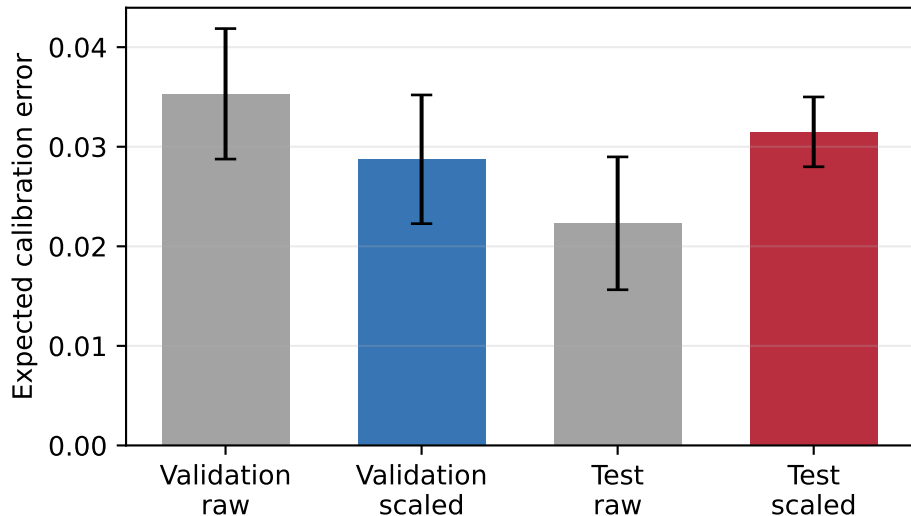
Temperature-scaling calibration effect
