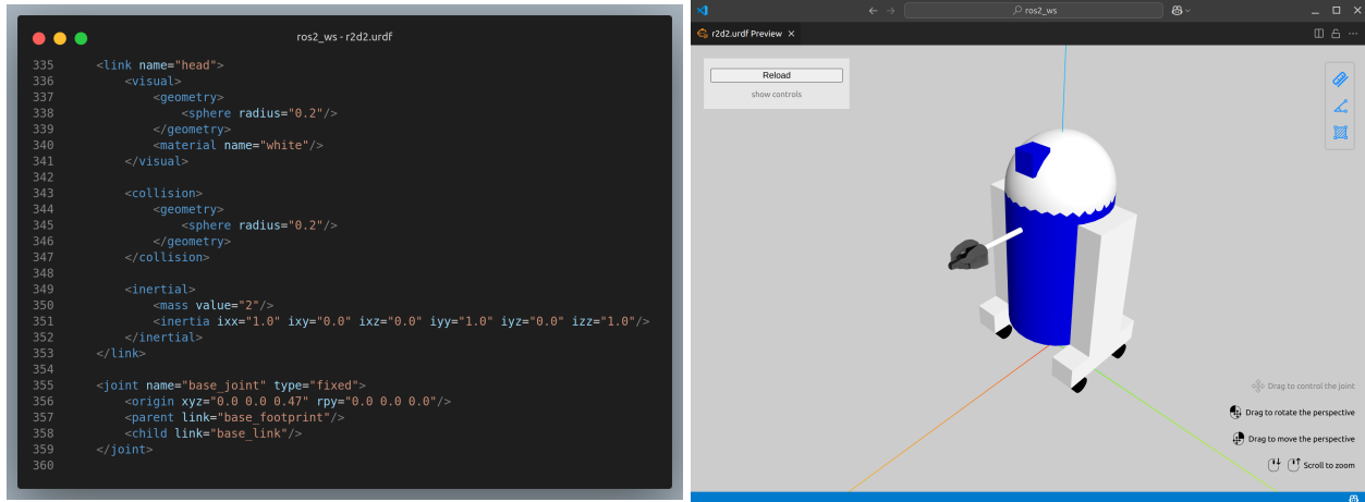
Figure 6.7: URDF modeling of a R2D2 using the URDF development and visualization extensions.
