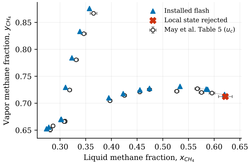
Methane liquid/vapor coexistence
