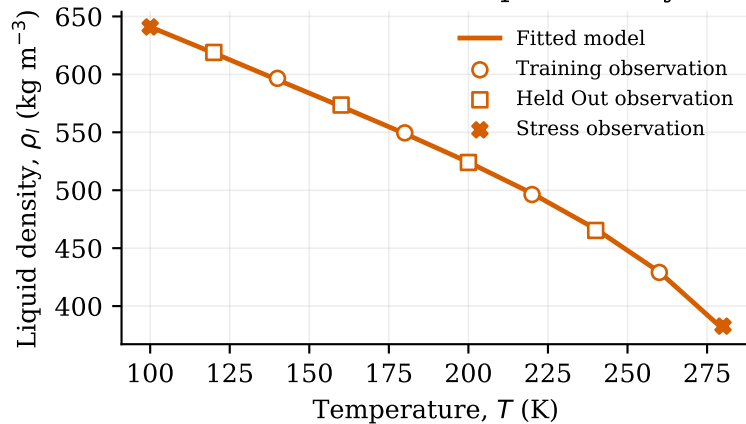
Ethane saturated-liquid density
