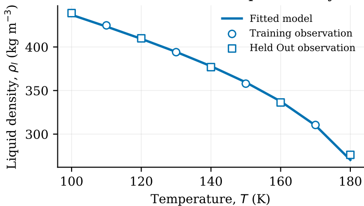
Methane saturated-liquid density
