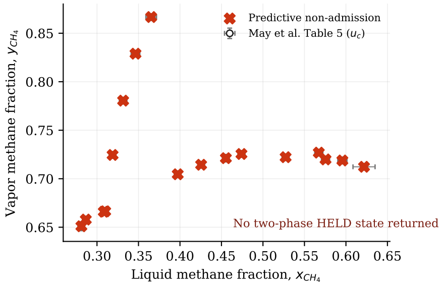
Methane/ethane coexistence
