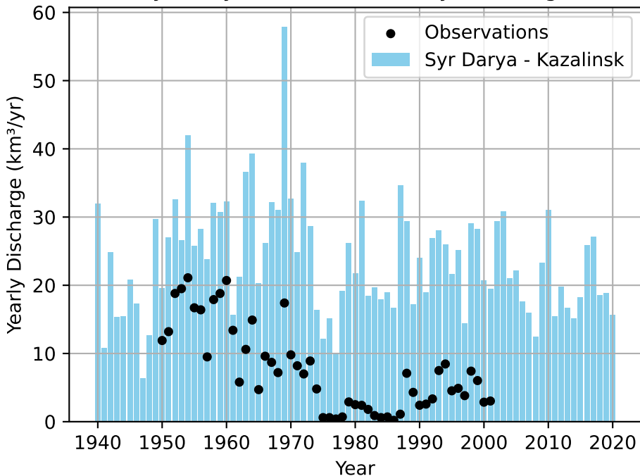
Syr Darya - Kazalinsk Yearly Discharge
