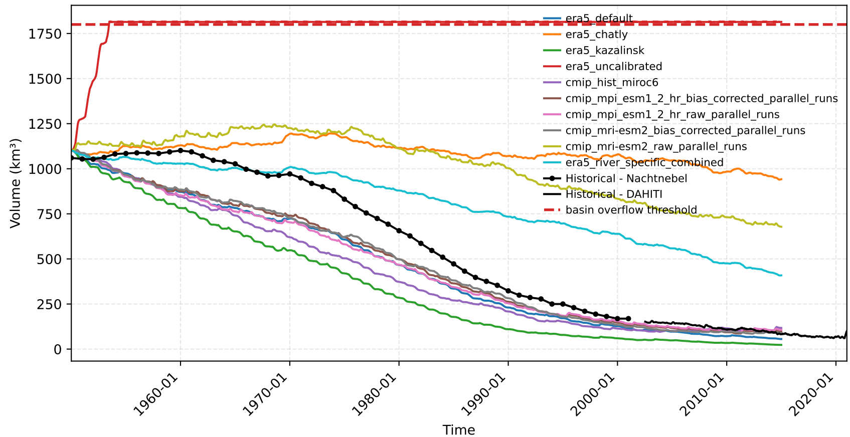
Aral Sea Volume
