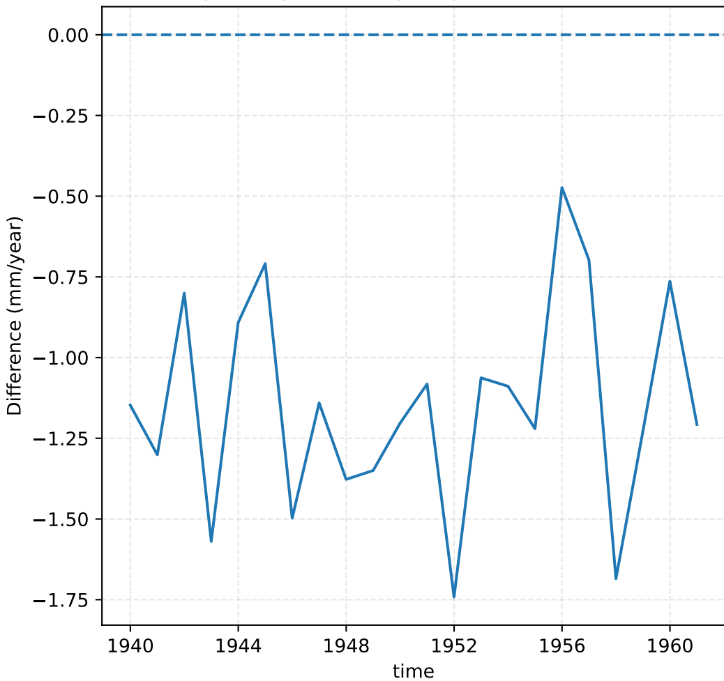
Regridding-induced precipitation difference
