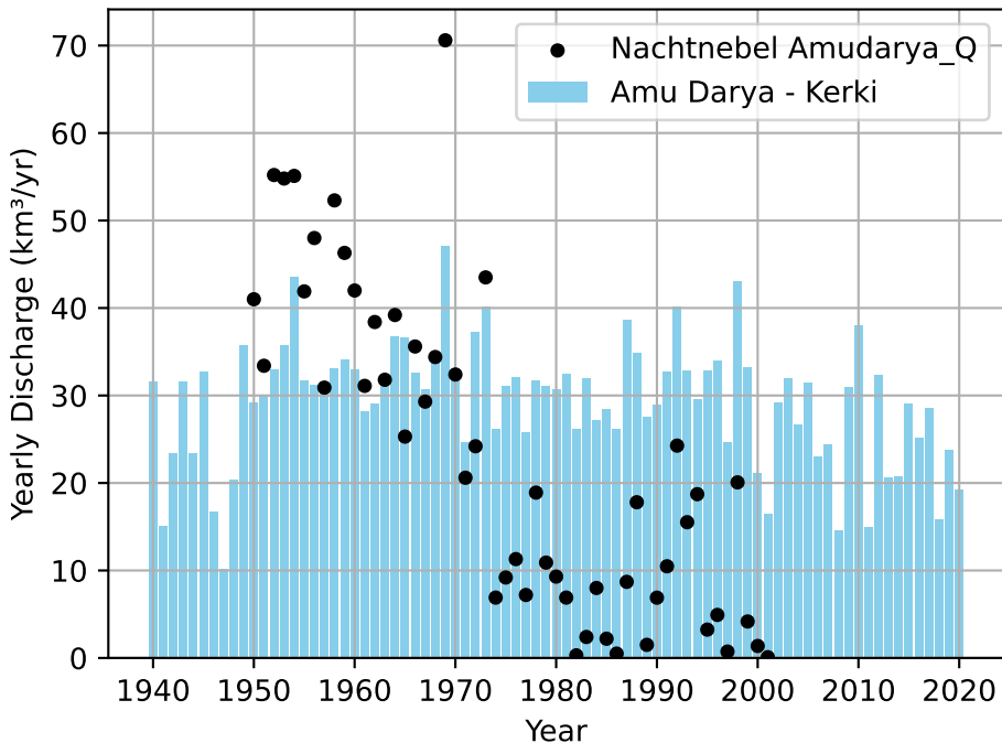
Amu Darya - Kerki Yearly Discharge
