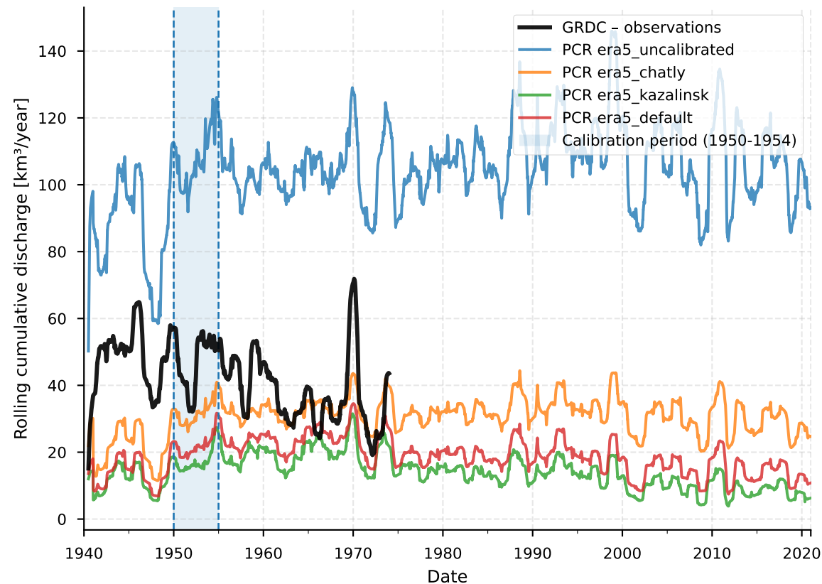
PCR-GLOBWB2 results: Chatly station
