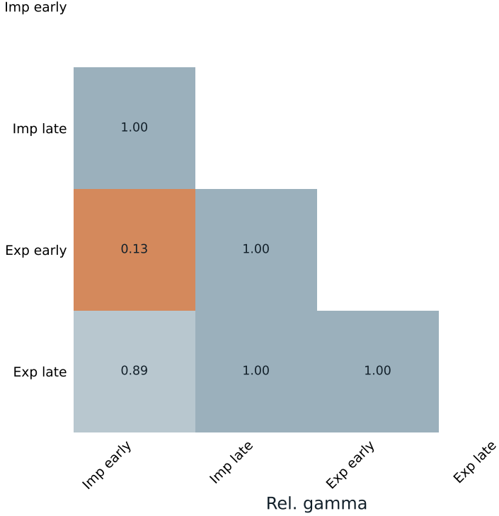
Rel. gamma
