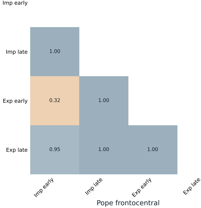
Pope frontocentral
