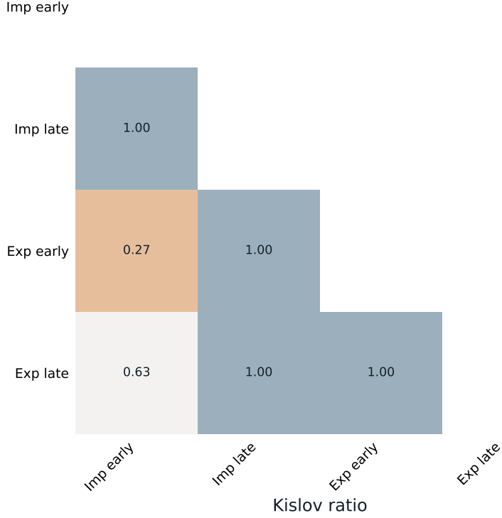
Kislov ratio
