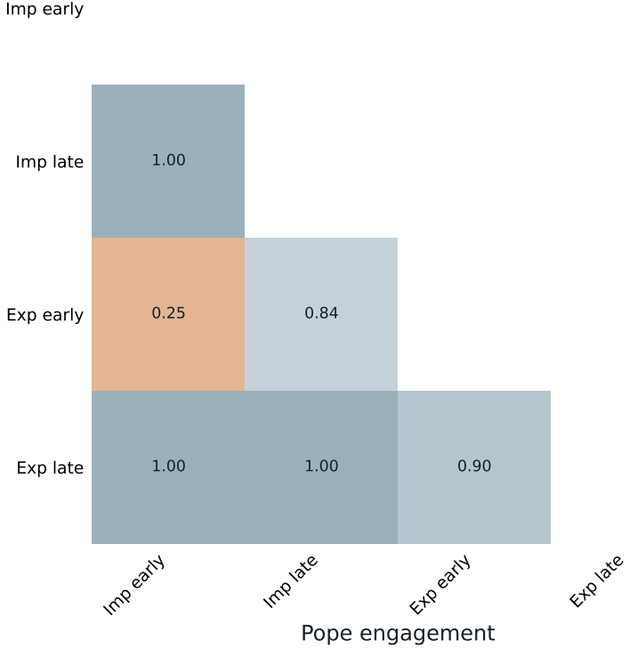
Pope engagement
