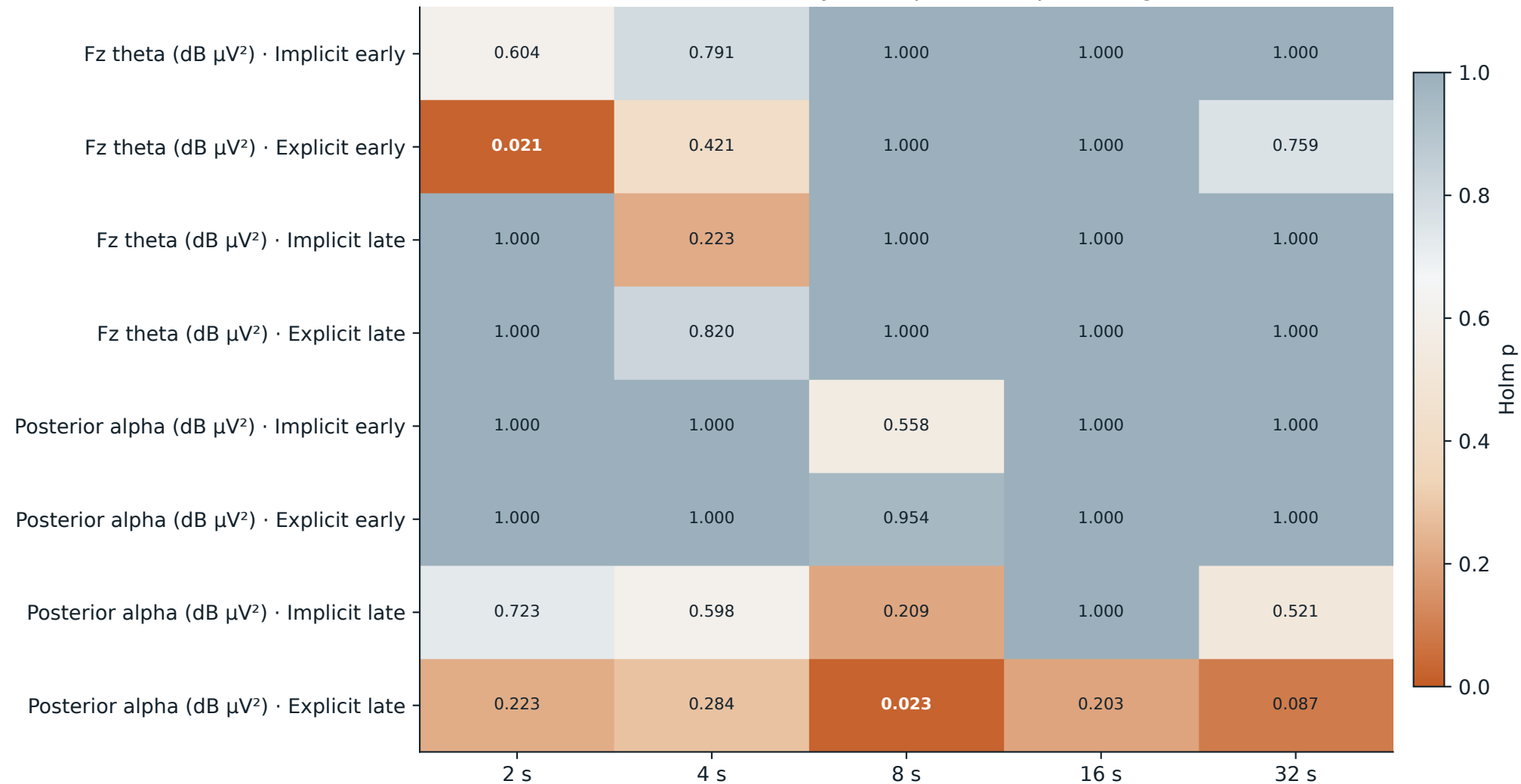
Dataset B confirmatory Holm p across epoch lengths (ICA)
