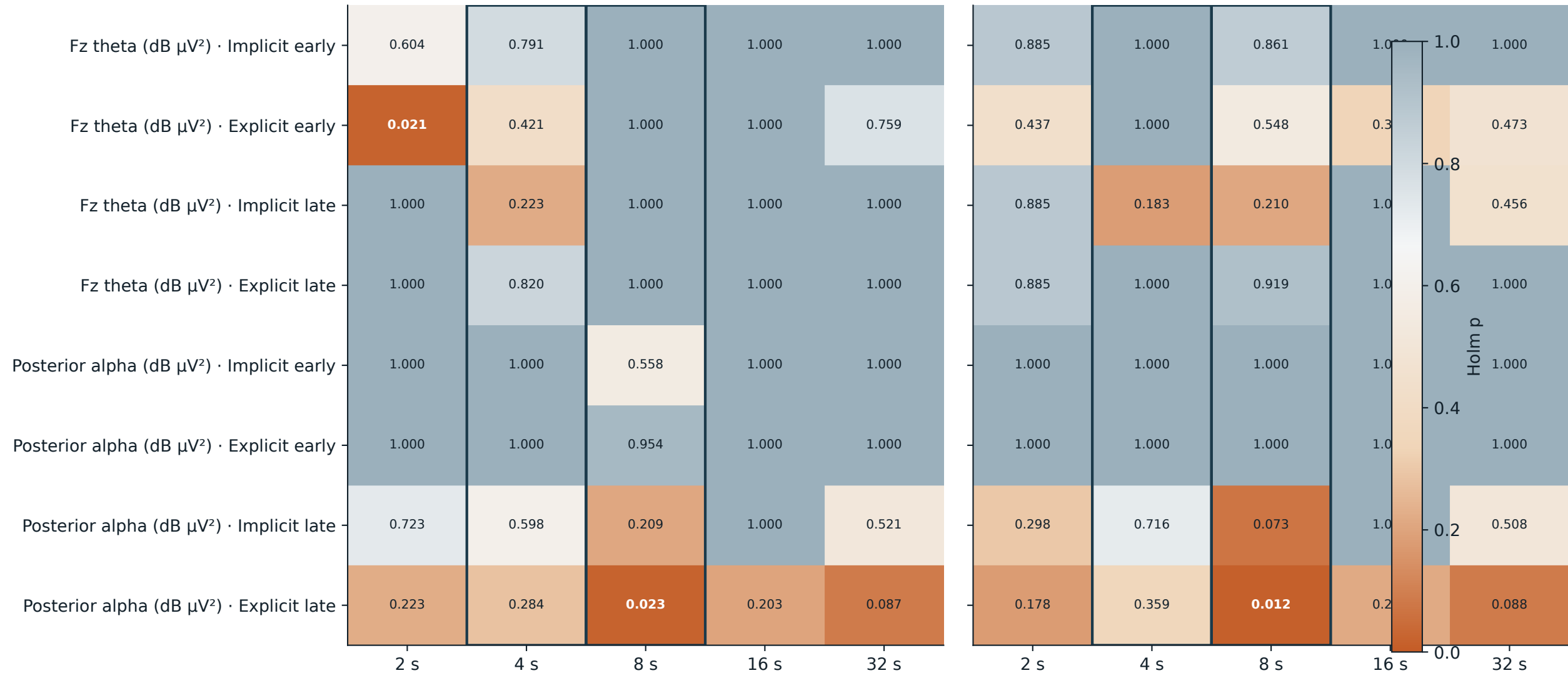
Dataset B confirmatory Holm p · ICA
