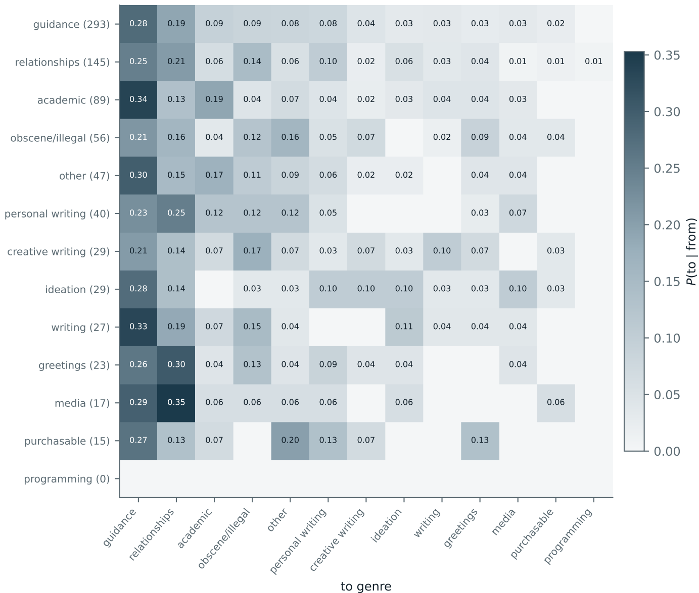
Row-normalised genre transition matrix
