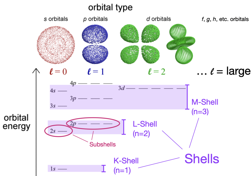
Figure 4.2: A diagram showing the orbital types for various electron configurations, quantized by the electron energy (principal quantum number n ) and orbital angular momentum (quantum number l ). This overall model, which includes orbital sizes that depend on a consideration of the electron spin, is also known as the Dirac model of the atom.
