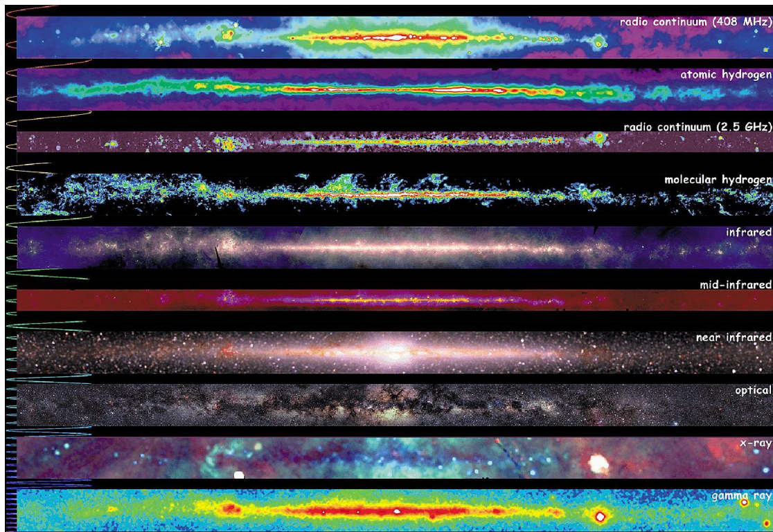
Figure 3.1: A multi-wavelength view of the plane of the Milky Way galaxy, showing the distribution of different components of the interstellar medium that can be seen with tracers at different wavelengths, including both line and continuum emission processes.
