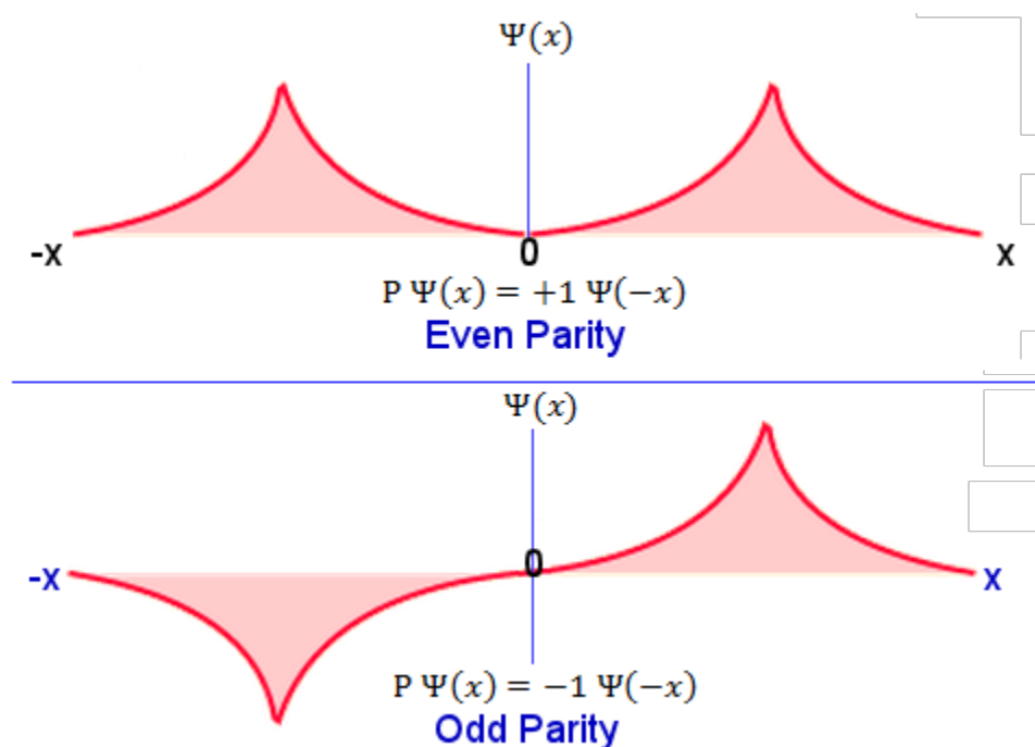
Figure 4.5: Even and odd parity wave functions, as defined by their symmetry (or lack thereof) when reflected across the y -axis.
