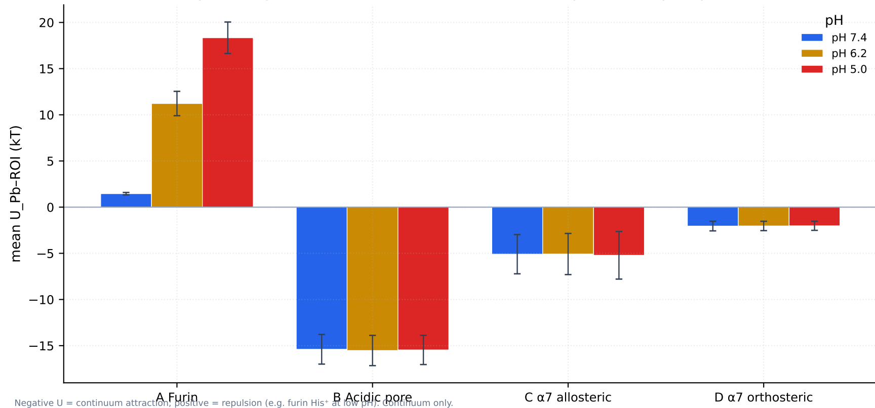
Fig 3 · Programme 1: exclusive \text{Pb}^{2+} across four public receptor proxies
