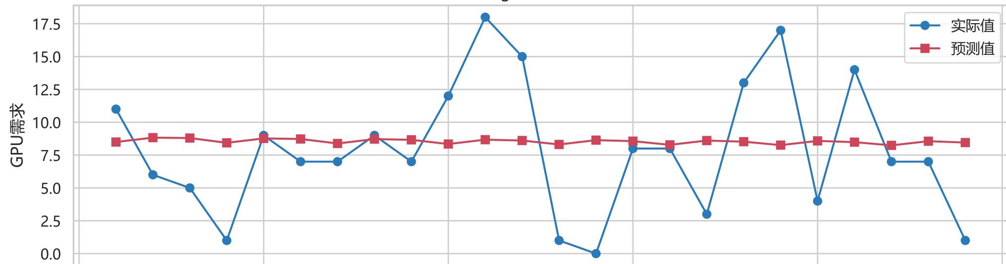
ARIMA示例: RegionB - RealTimeInference
