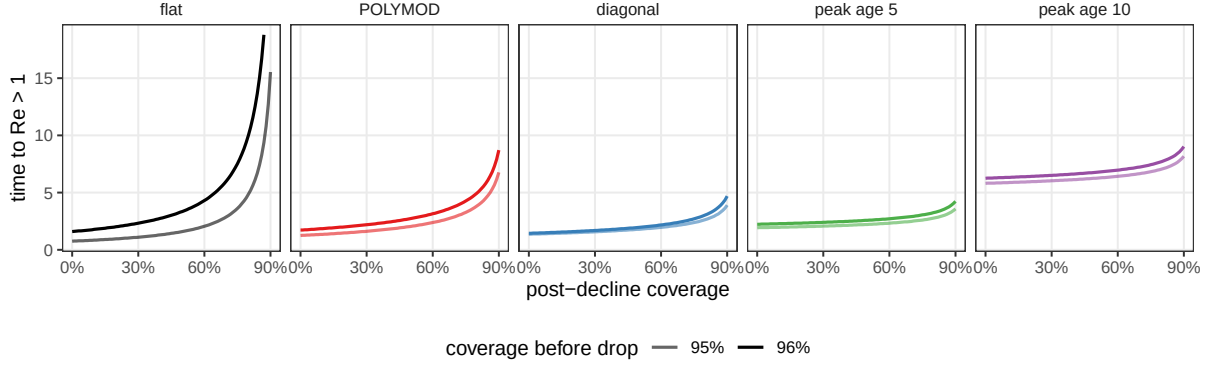
Figure S2: Theoretical honeymoon time predictions, computed as time until Re \geq 1 , under five assumptions about age-structured mixing. Results are shown for a population with \mu = 1/80 \text{ years}^{-1} , a pathogen with R_0 = 17 , and a pre-decline immunization of 95% and 96%.
