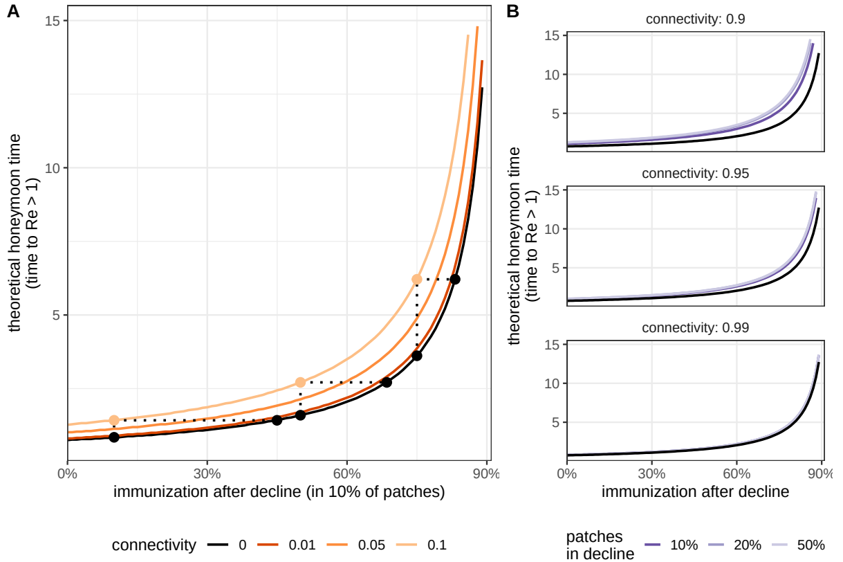
Figure S3: Role of patch connectivity in theoretical honeymoon time. (A) Theoretical honeymoon time, computed as time until Re \geq 1 , by post-decline immunization when drops occur in 10% of patches among an equally connected network. Line color shows connectivity between patches (where 0.05 indicates 5% of transmission is shared between patches, or c above), and the points show equivalence between a model with no connectivity and a model where 10% of transmission is shared between patches. (B) Sensitivity of results to the percent of patches in which immunization declines, or \rho above. Results are shown for a population with \mu = 1/80 \text{ years}^{-1} , a pathogen with R_0 = 17 , and a pre-decline immunization of 95%.
