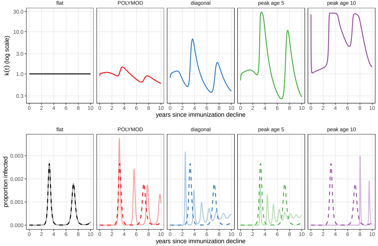
Figure S2: Illustration of k(t) for five example WAIFW matrices. (A) Equivalence ratio, k(t) , scales age-structured transmission to yield dynamics equivalent to the homogeneous model. When k(t) < 1 , unscaled transmission in the age-structured model is higher than the homogeneous model, indicating that age-structure would have “sped up” dynamics; vice versa when k(t) > 1 . (B) Infection dynamics since immunization decline in the age-structured model under different WAIFW matrices are shown in the light solid lines (equivalent to Main text Figure 3), and dashed lines show infection dynamics when k(t) is used to scale transmission in the age-structured model. See Main text for details on sample WAIFW matrices.
