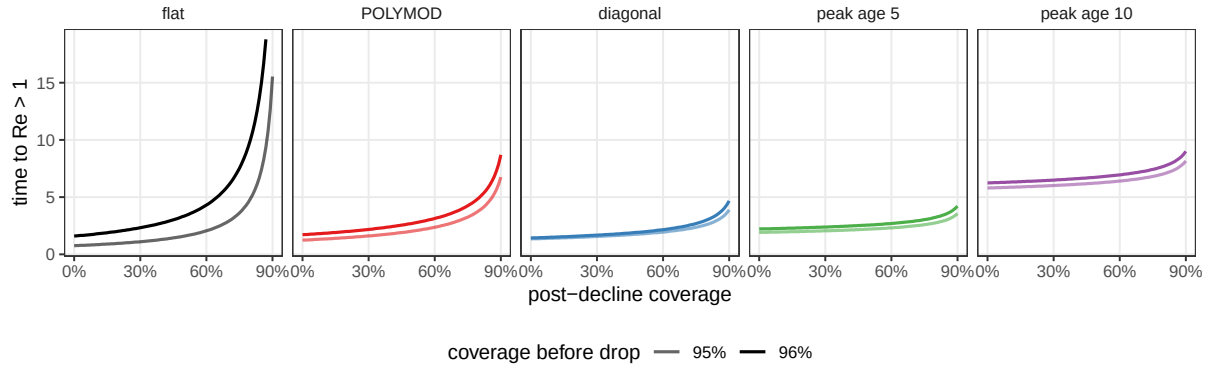
Figure S4: Theoretical honeymoon time predictions, computed as time until \mathcal{R}_{\text{eff}} > 1 , under five assumptions about age-structured mixing. Results are shown for a population with \mu = 1/80 \text{ years}^{-1} , a pathogen with \mathcal{R}_0 = 17 , and pre-decline effective immunization coverage of 95% and 96%.
