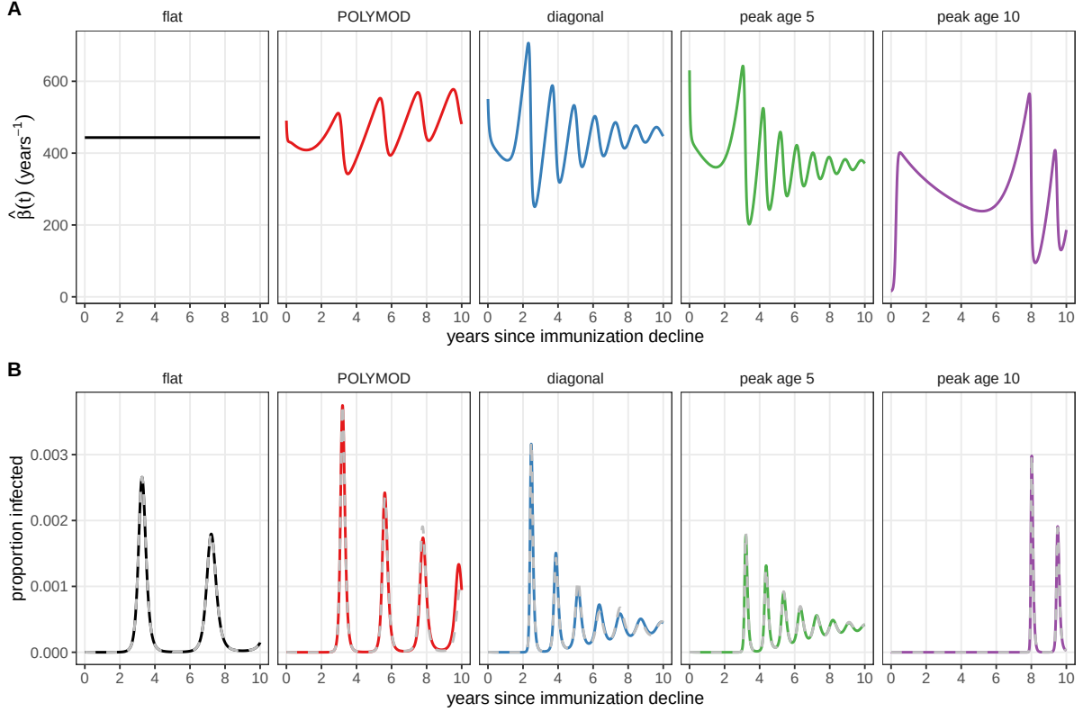
Figure S1: Illustration of \hat{\beta}(t) for five sample WAIFW matrices. (A) Time-varying transmission rate, \hat{\beta}(t) , scales homogeneous dynamics to age-structured. The flat line for the flat matrix is the annual transmission rate that yields \mathcal{R}_0 = 17 given \gamma = 1/14 days -1 and \mu = 1/80 years -1 . (B) Infection dynamics since immunization decline in the age-structured model under different WAIFW matrices are shown in the solid colored lines (equivalent to Main text Figure 3), and the dashed gray lines (overlaid) show infection dynamics in a homogeneous model with time-varying transmission rate, \hat{\beta}(t) . See Main text for details on sample WAIFW matrices.
