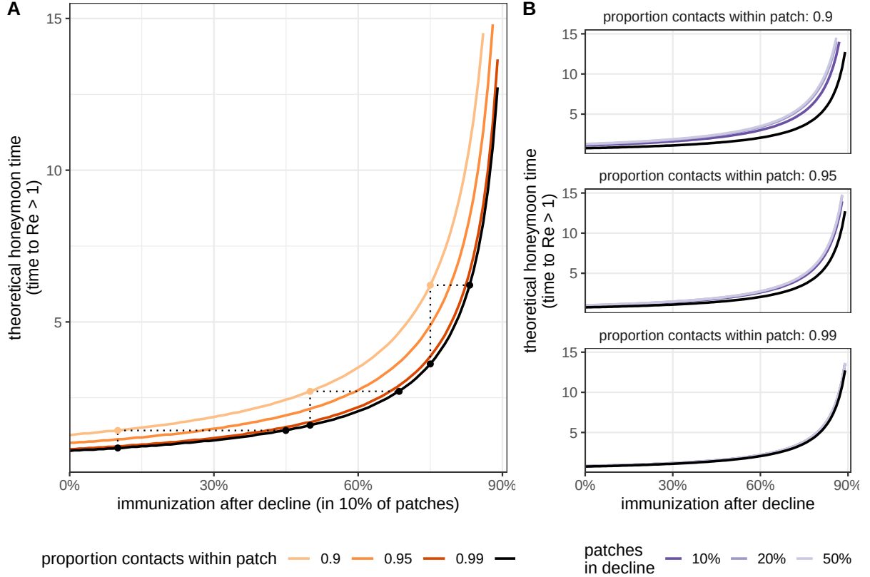
Figure S5: Role of patch connectivity in theoretical honeymoon time. (A) Theoretical honeymoon time, computed as time until \mathcal{R}_{\text{eff}} > 1 , by post-decline effective immunization coverage when drops occur in 10% of patches among an equally connected network. Line color shows different connectivity scenarios, modeled by the proportion of contacts that occur within the home patch, and the points show equivalence between a model with no connectivity (i.e., 100% of contacts occurring within the home patch) and a model where 90% of contacts occur within the home patch. (B) Sensitivity of results to the percent of patches in which effective immunization coverage declines compared to the no connectivity scenario (black). Results are shown for a population with \mu = 1/80 \text{ years}^{-1} , a pathogen with \mathcal{R}_0 = 17 , and pre-decline effective immunization coverage of 95%.
