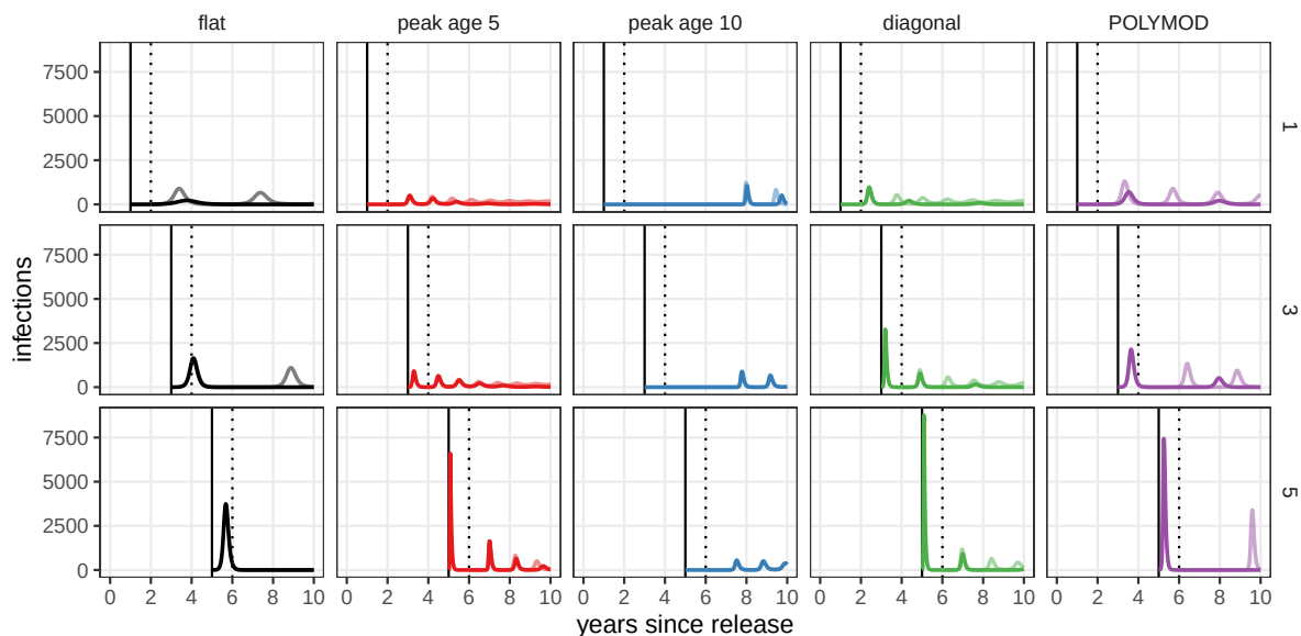
Figure S3: Sensitivity of results to the timing of infection introduction. For each WAIFW matrix (columns, see main text Figure 3A), simulated dynamics when a single infection is introduced into the 5 year old age class 1, 3, or 5 years after the drop in effective immunization coverage (rows). The solid vertical line shows the timing of introduction. The lighter line shows simulation results if effective immunization coverage returns to its pre-decline level 1 year after the drop (shown by dotted line).
