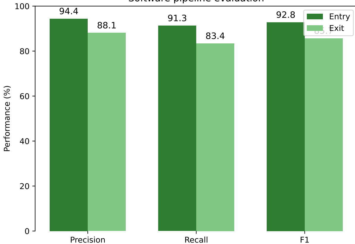
Software pipeline evaluation
