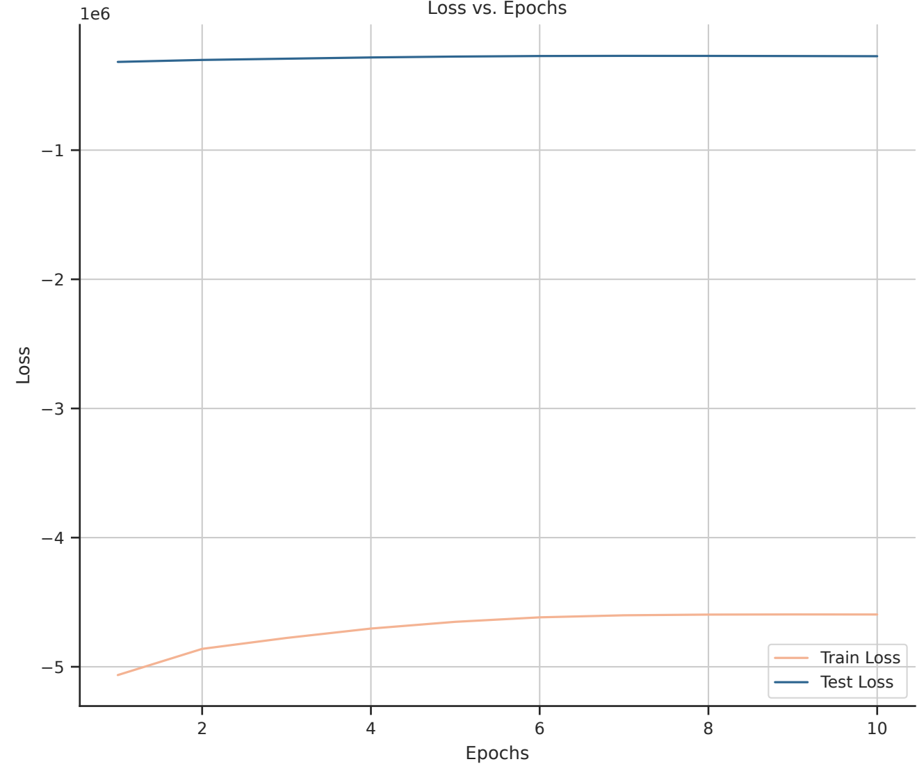
Loss vs. Epochs
