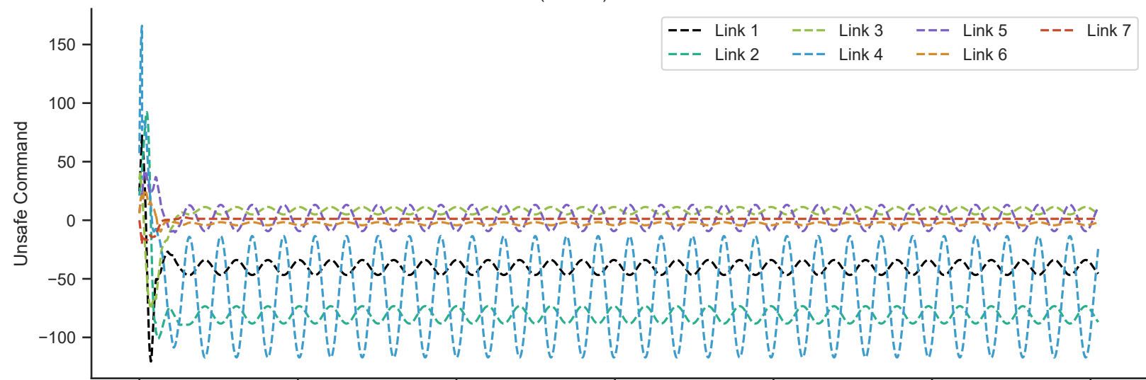
Nominal (Unsafe) Control Commands
