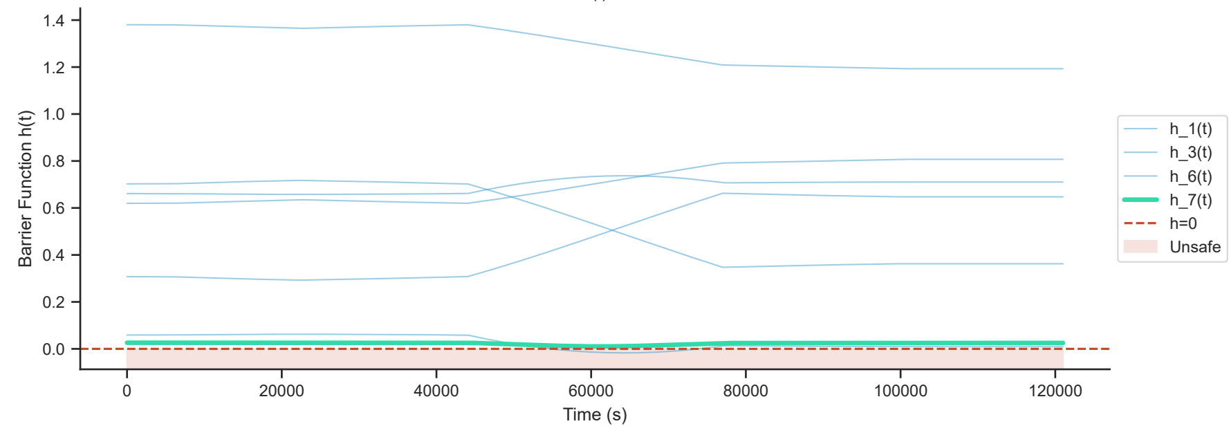
Barrier Function h(t) Over Simulation
