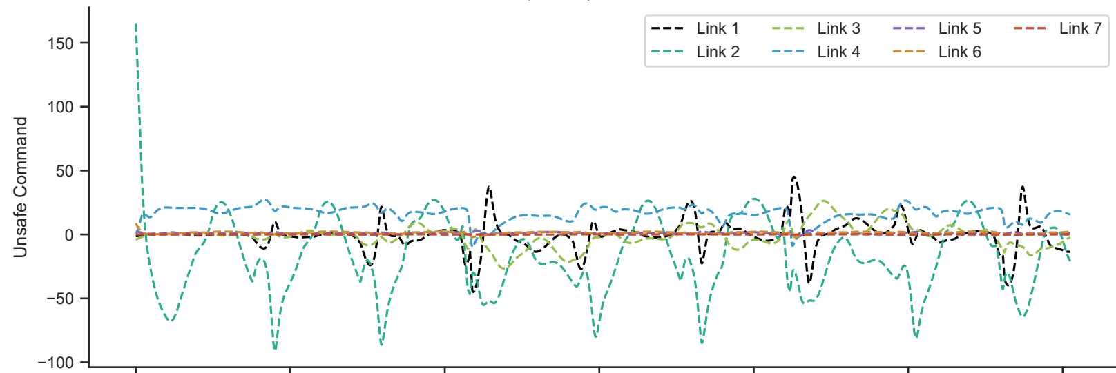
Nominal (Unsafe) Control Commands
