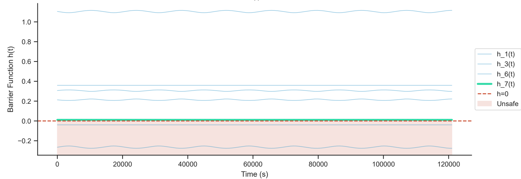
Barrier Function h(t) Over Simulation
