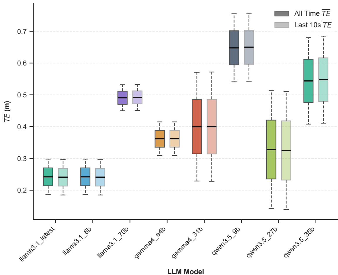
Multiple Safety Conditions Example (prompt v1.5) - \overline{TE}
