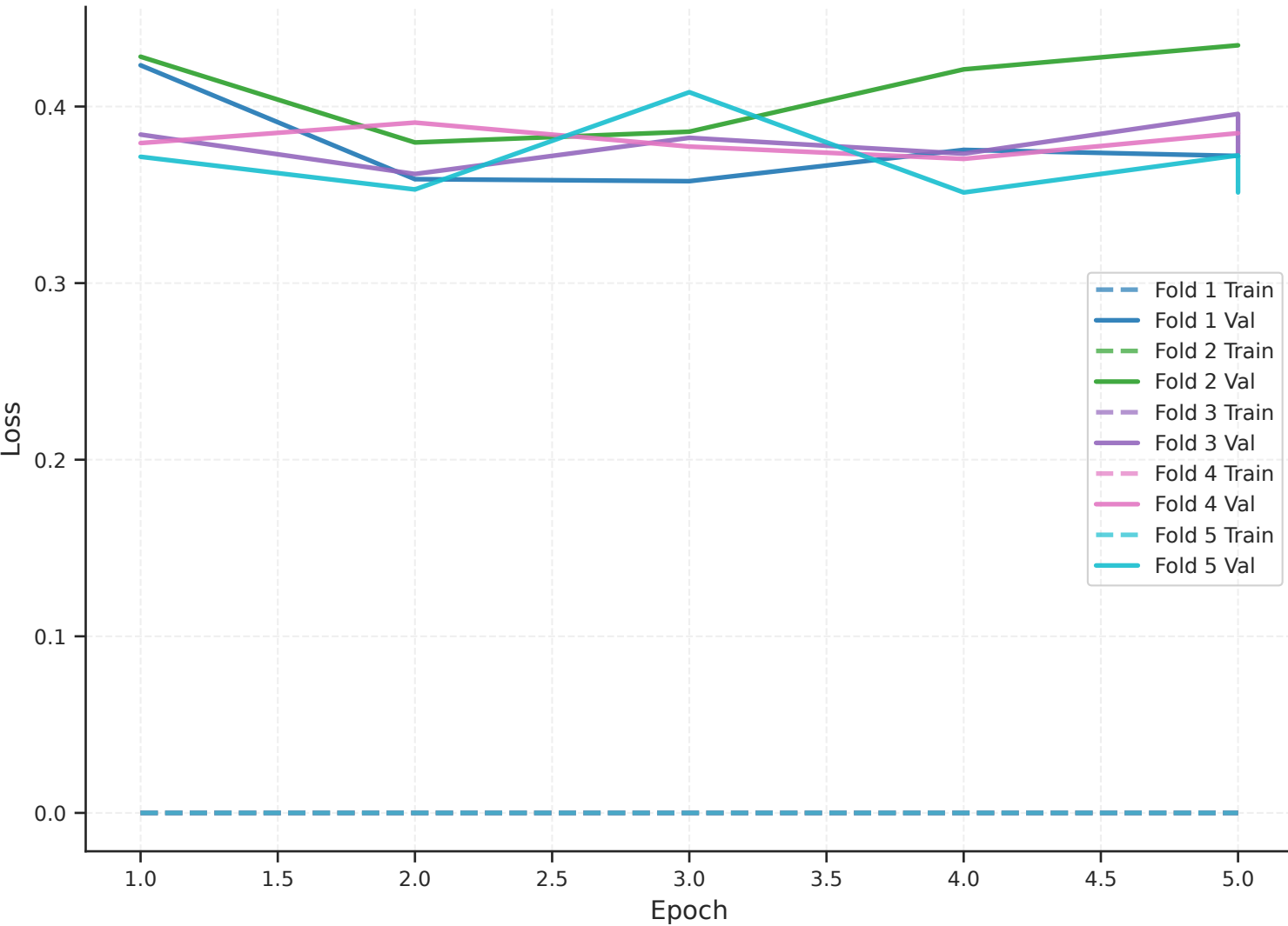
Training & Validation Loss - deberta-v3-base
