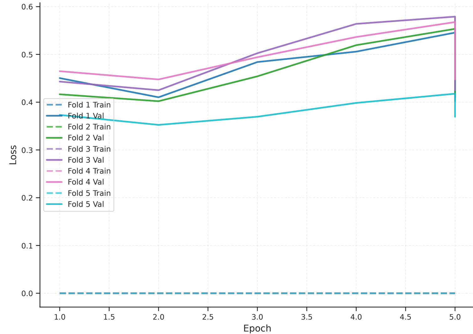
Training & Validation Loss - twitter-roberta-base-hate-latest
