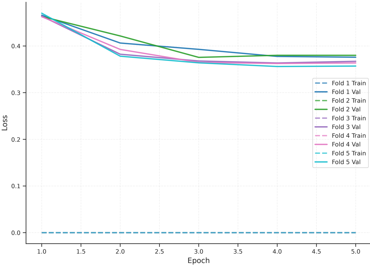
Training & Validation Loss - twitter-roberta-base-2022-154m
