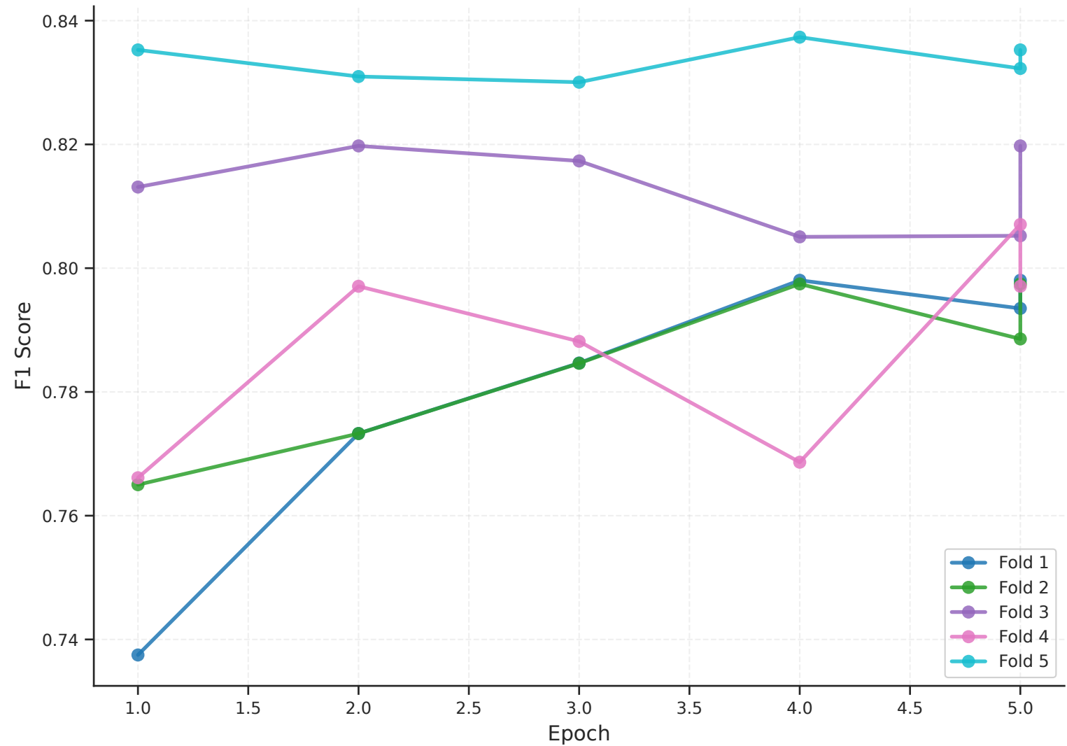
F1 Macro Score - twitter-roberta-base-sentiment-latest
