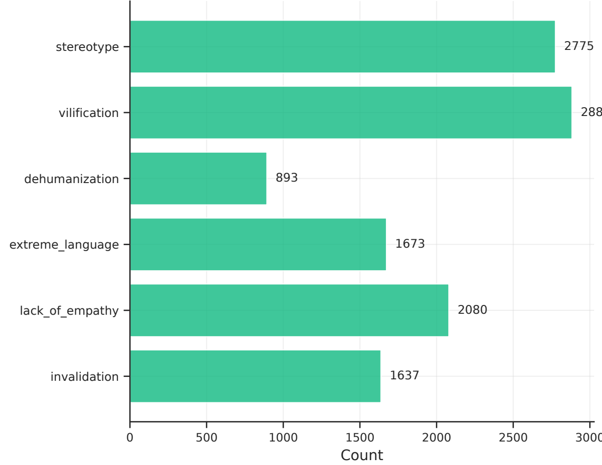
Swahili Train
