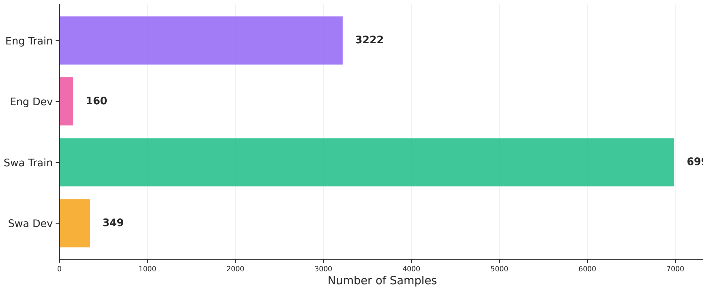
Dataset Sizes
