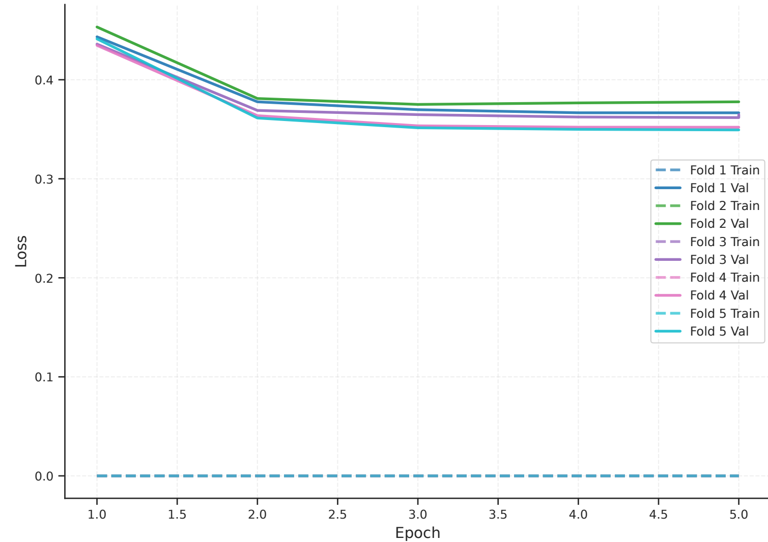
Training & Validation Loss - twitter-roberta-base-hate-multiclass-latest
