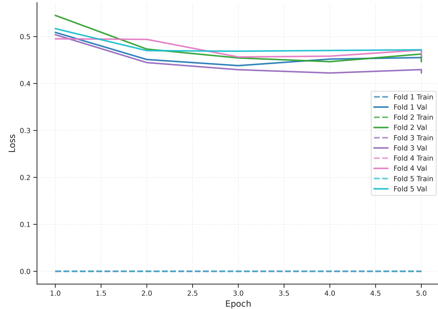
Training & Validation Loss - afro-xlmr-base
