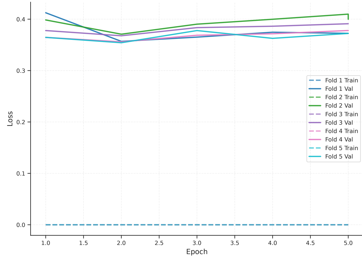
Training & Validation Loss - twitter-roberta-base-sentiment-latest
