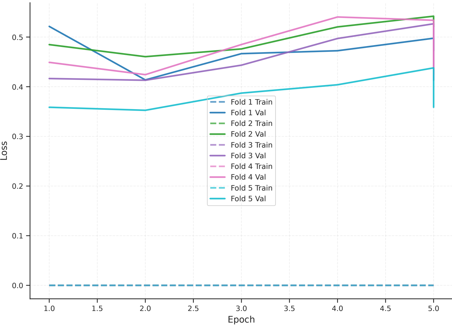
Training & Validation Loss - twitter-roberta-base-sentiment-latest
