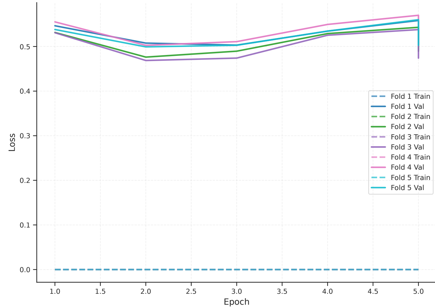
Training & Validation Loss - swahBERT
