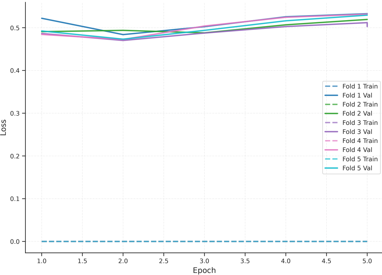
Training & Validation Loss - swahBERT
