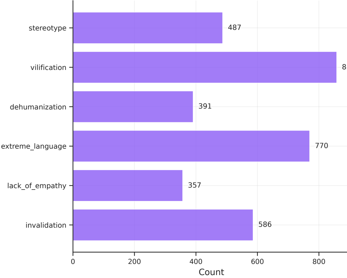
English Train
