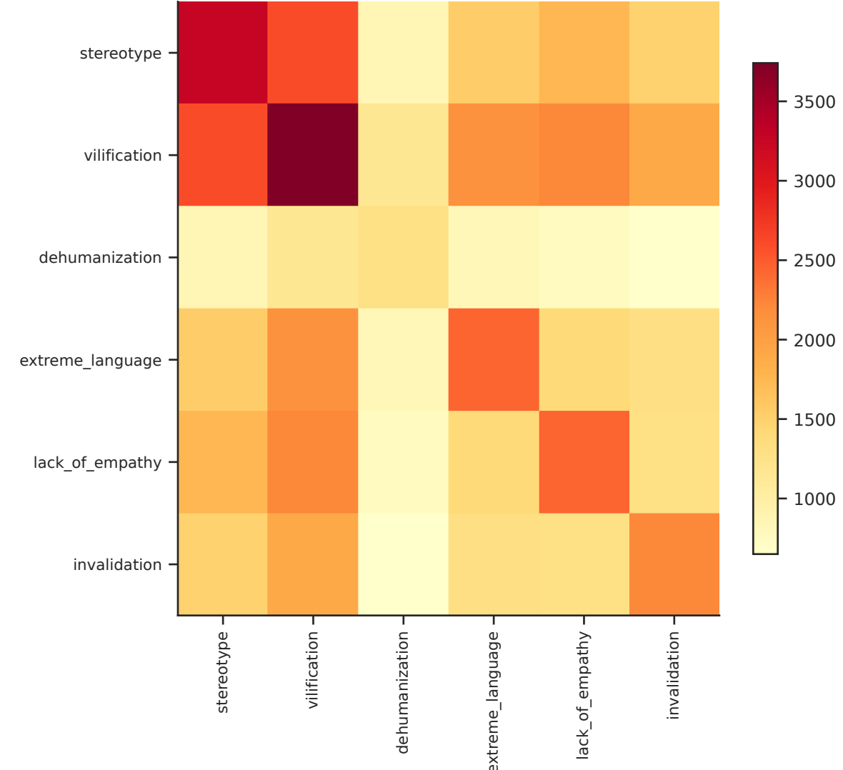
Label Co-occurrence
