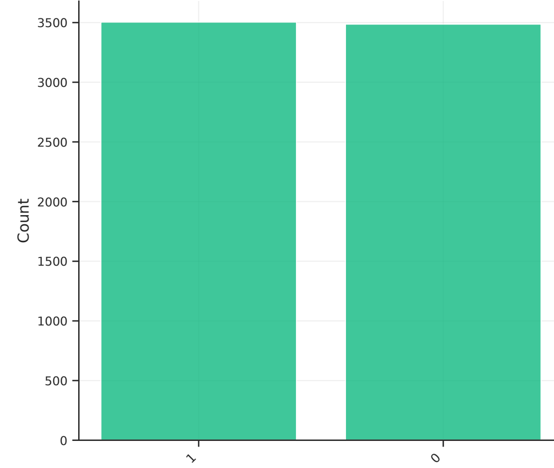
Swahili Train
