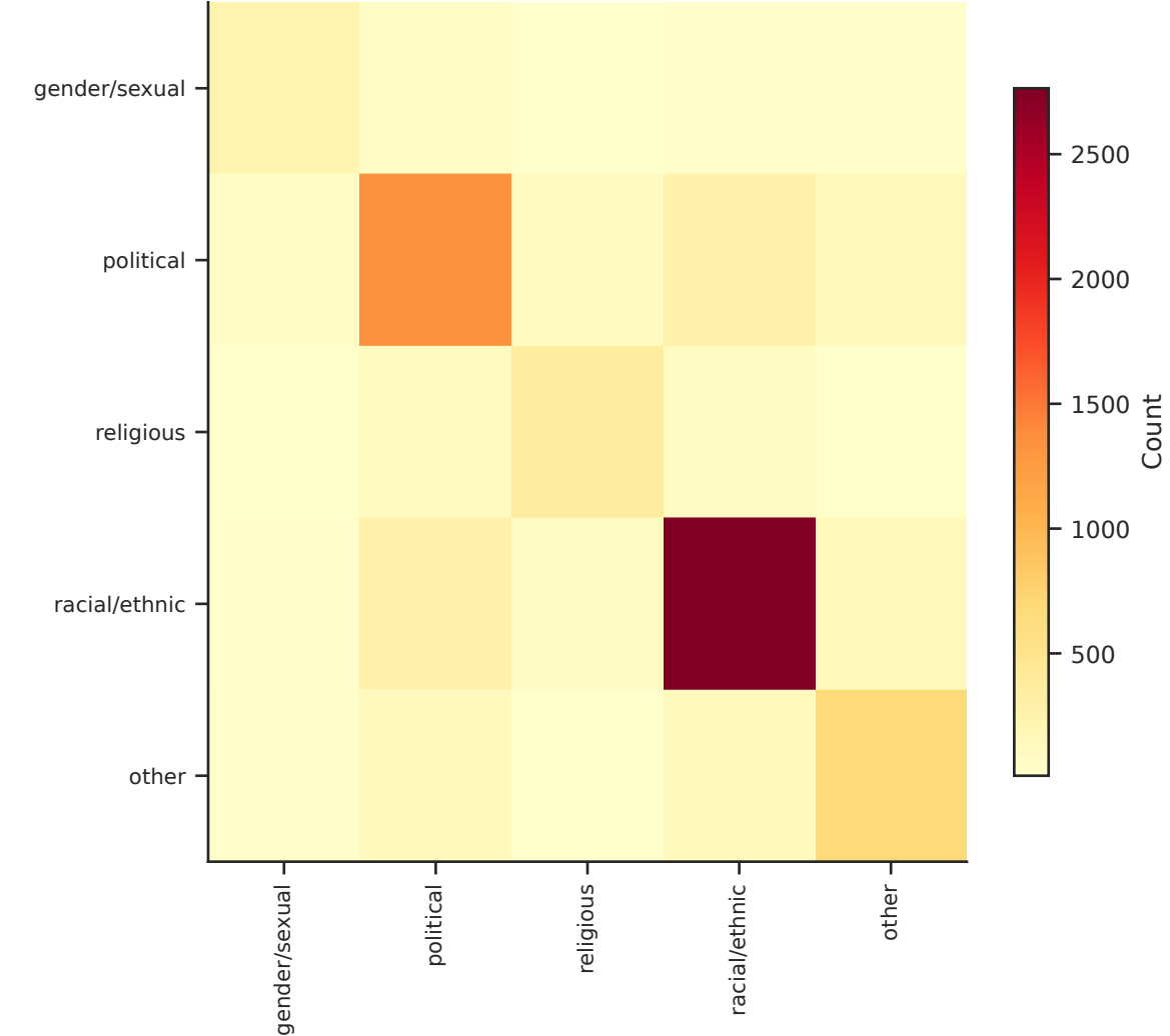
Label Co-occurrence
