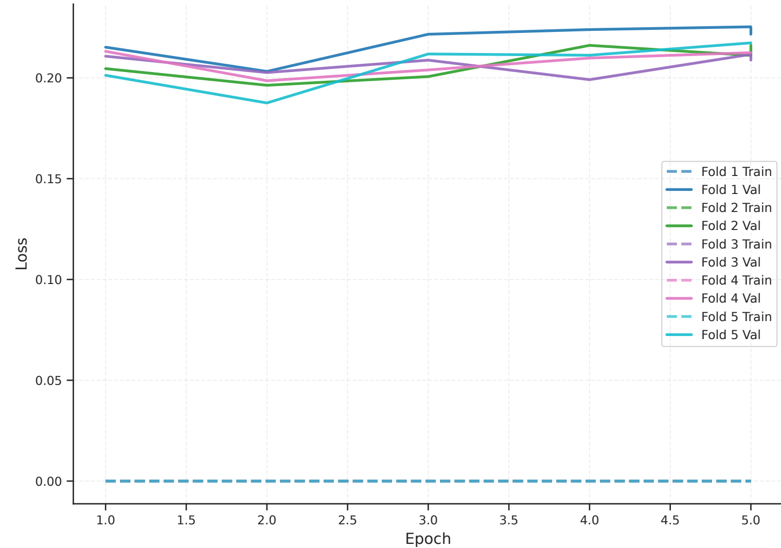
Training & Validation Loss - twitter-roberta-base-hate-multiclass-latest
