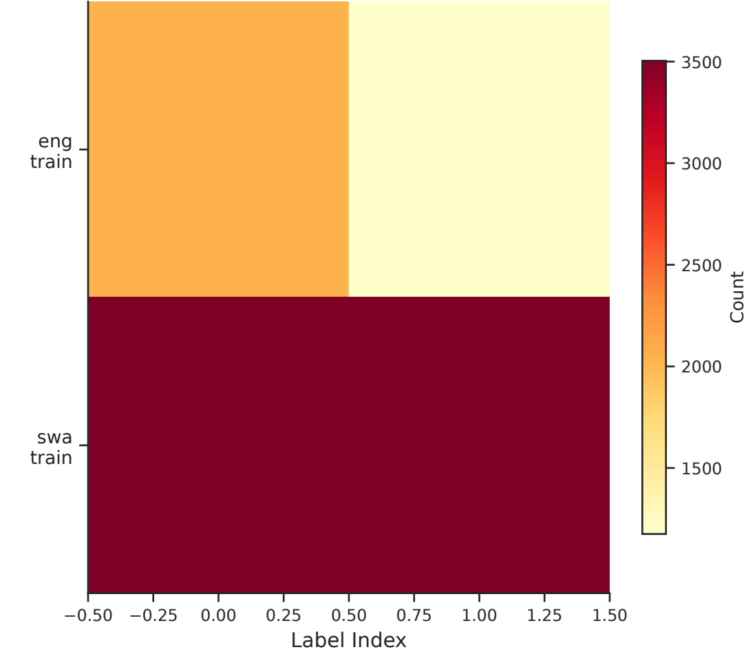
Class Balance
