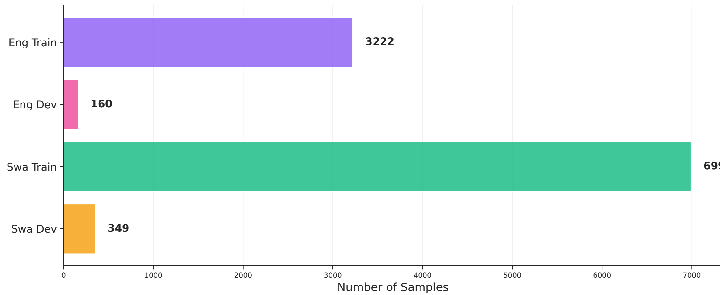
Dataset Sizes
