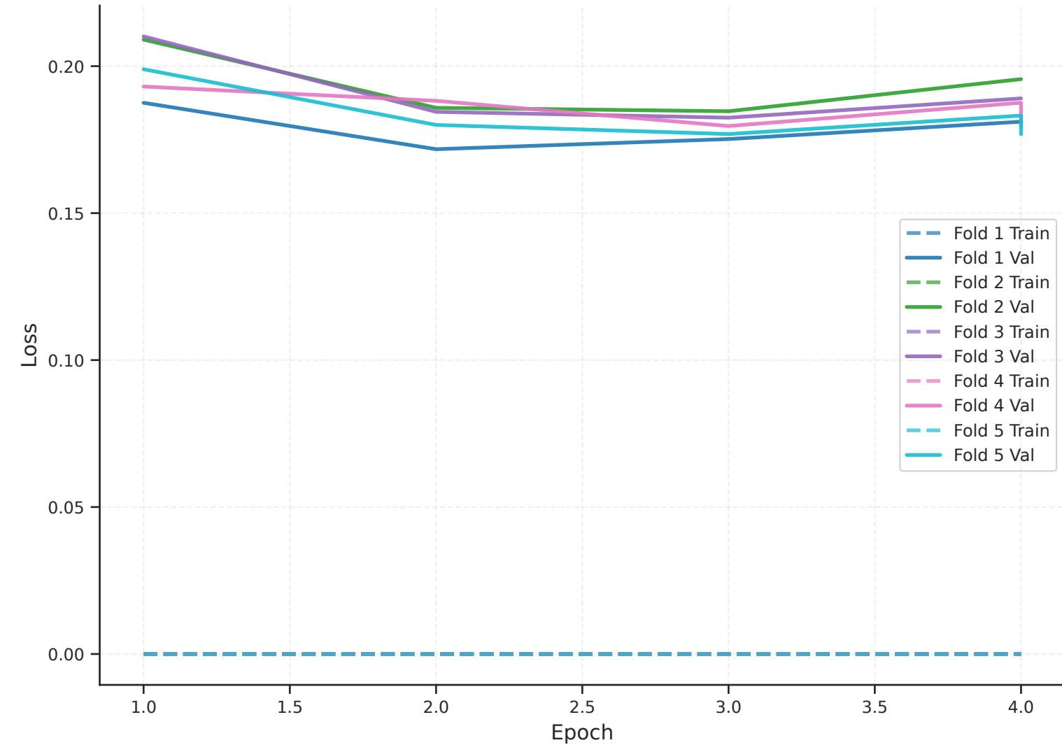
Training & Validation Loss - swahBERT
