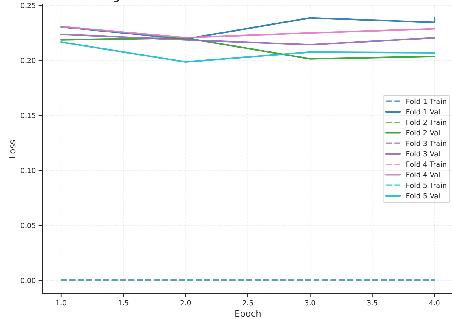
Training & Validation Loss - twitter-xlm-roberta-base-sentiment
