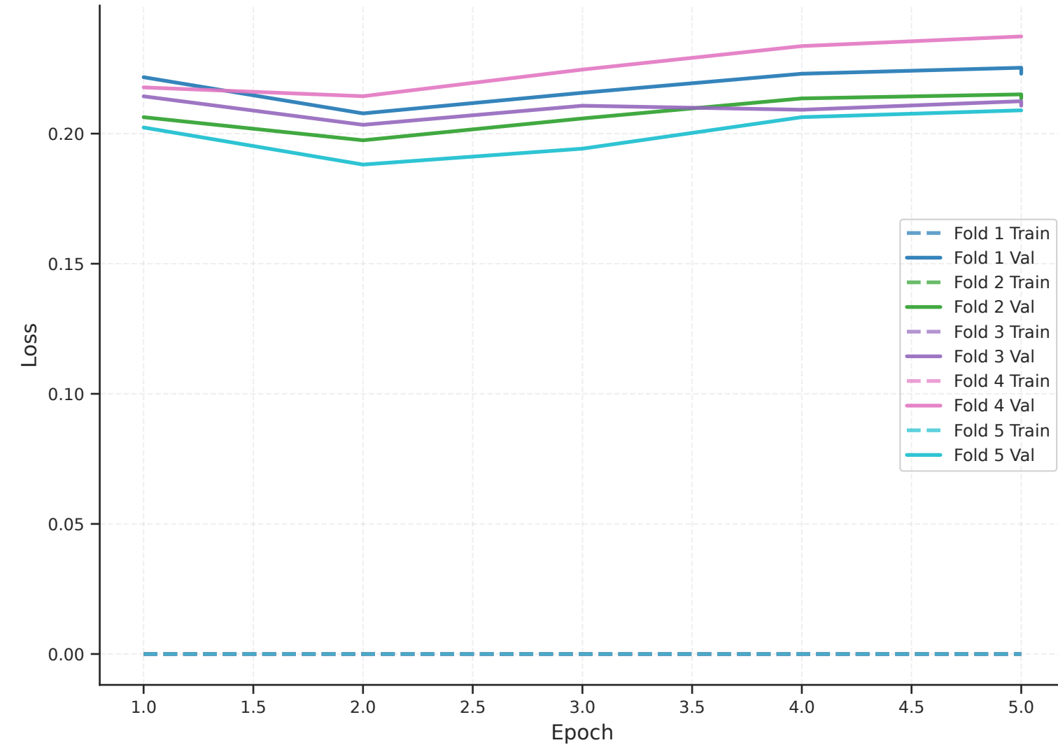
Training & Validation Loss - twitter-roberta-base-hate
