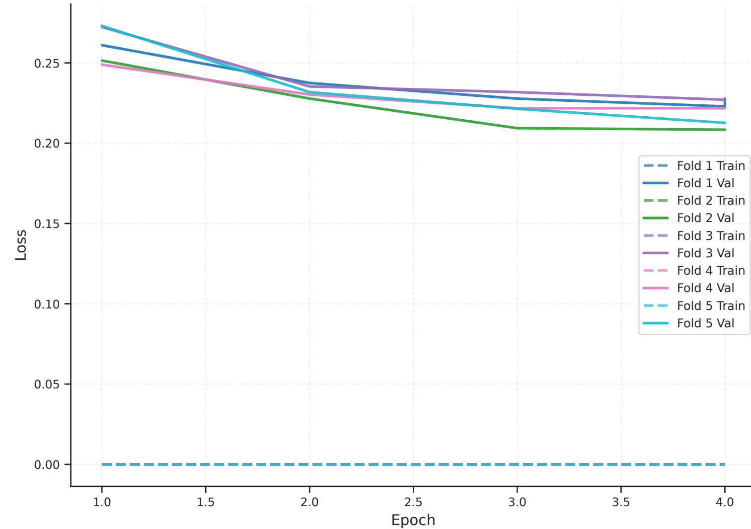
Training & Validation Loss - xlm-roberta-base
