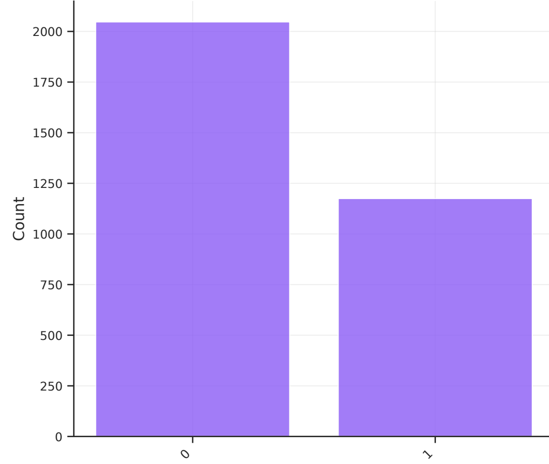
English Train
