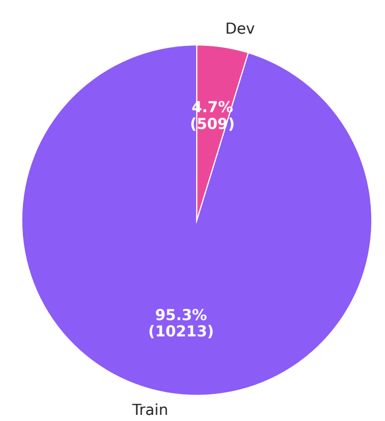
Train/Dev Split
