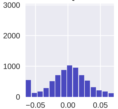
Normalized Quantization
