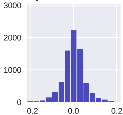
Quantization Aware
