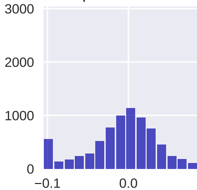
Proposed Method
