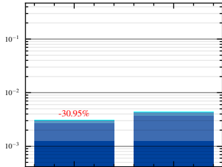
LeNet5
