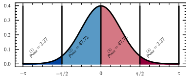
Density distribution for \tau = 4
