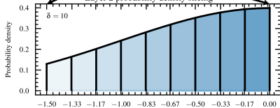
Layer 2 probability density slicing
