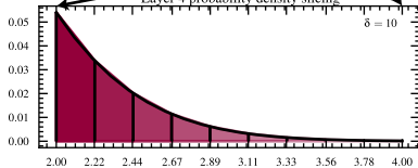
Layer 4 probability density slicing
