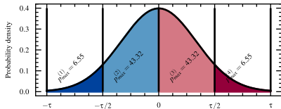
Density distribution for \tau = 3
