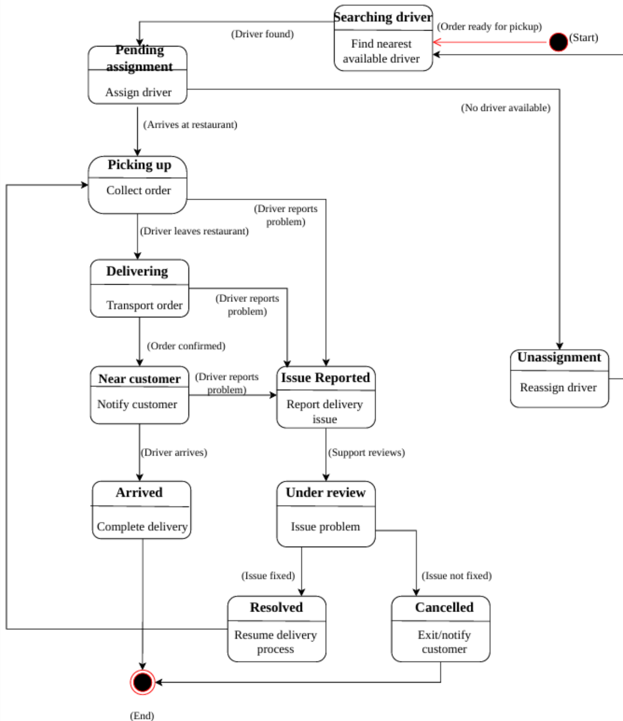
State Diagram 3- Delivery State Diagram
