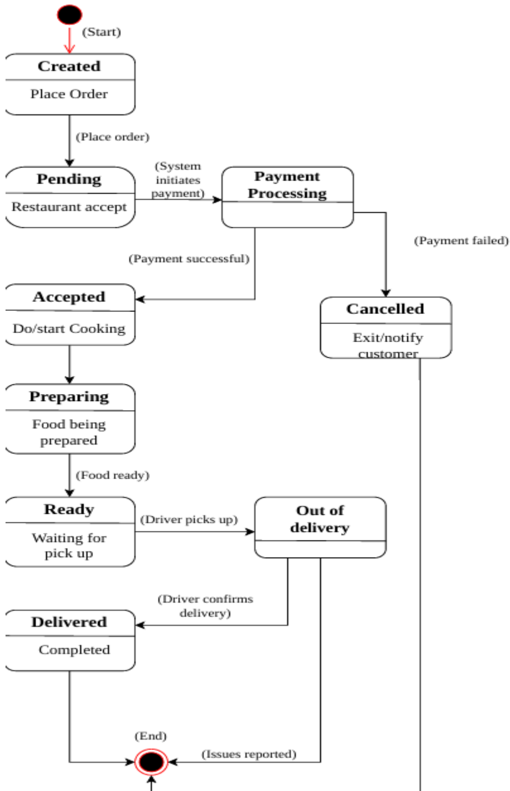
State Diagram 1- Order State Diagram
