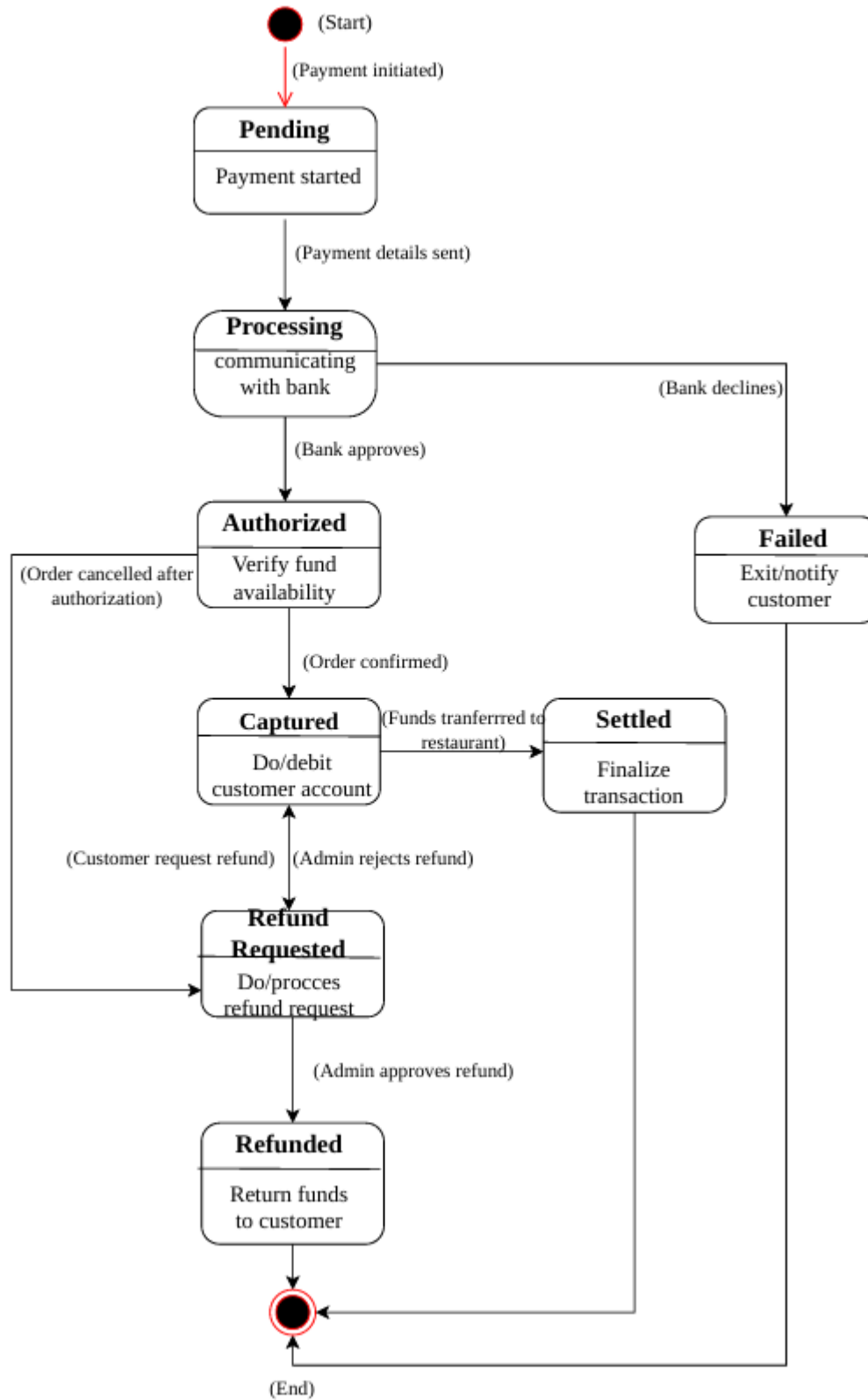
State Diagram 2- Payment State Diagram
