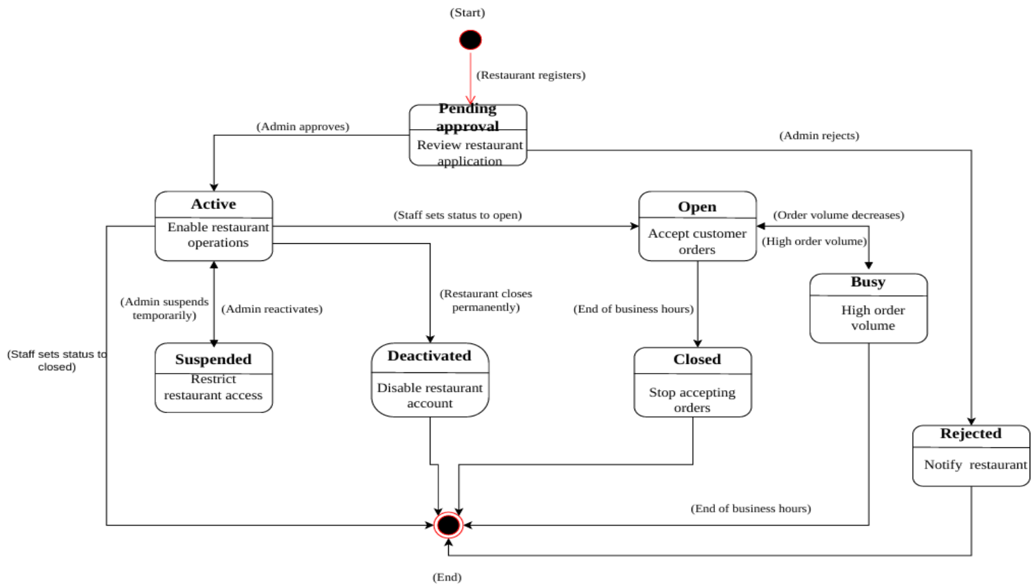
State Diagram 4- Restaurant Status State Diagram
