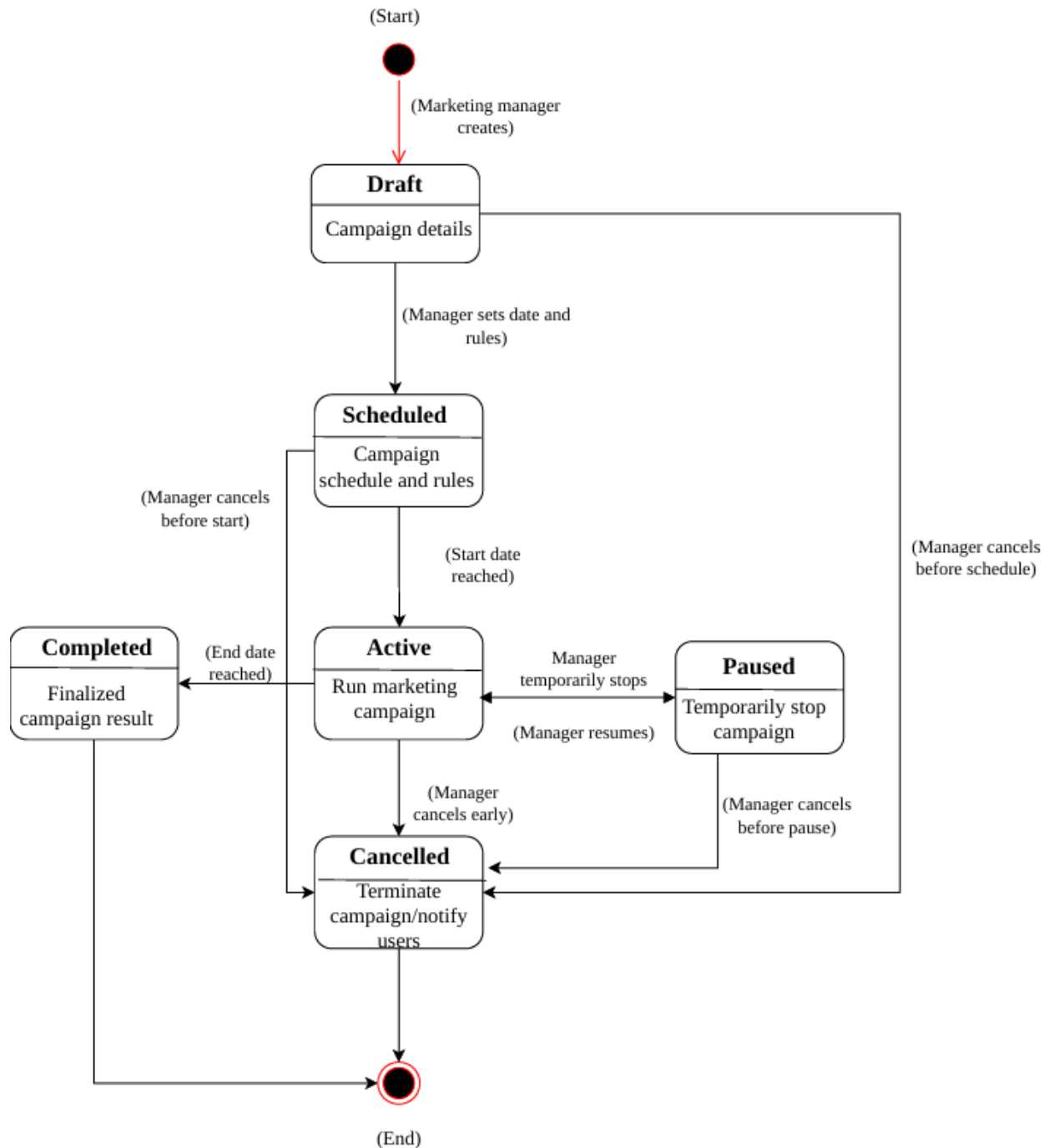
State Diagram 6- Marketing Campaign State Diagram
