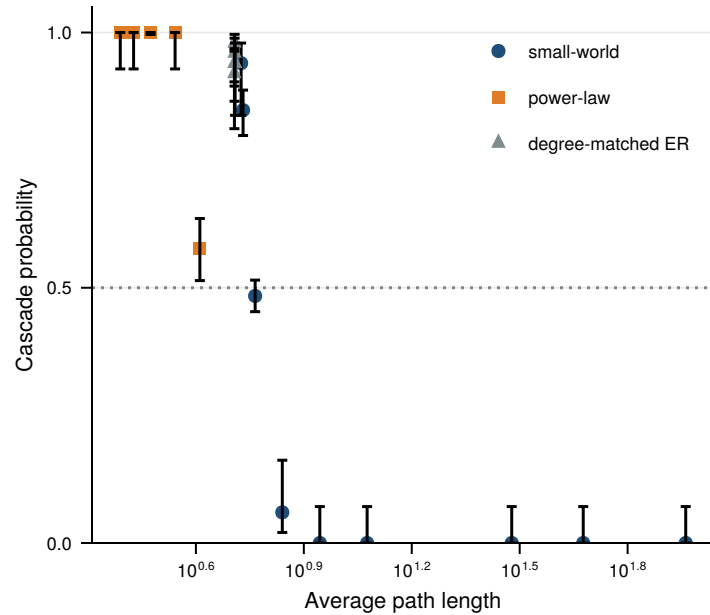
(c) Cascades need short paths
