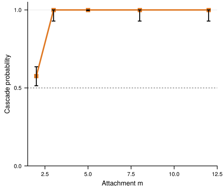
(b) Power-law: cascades at low m
