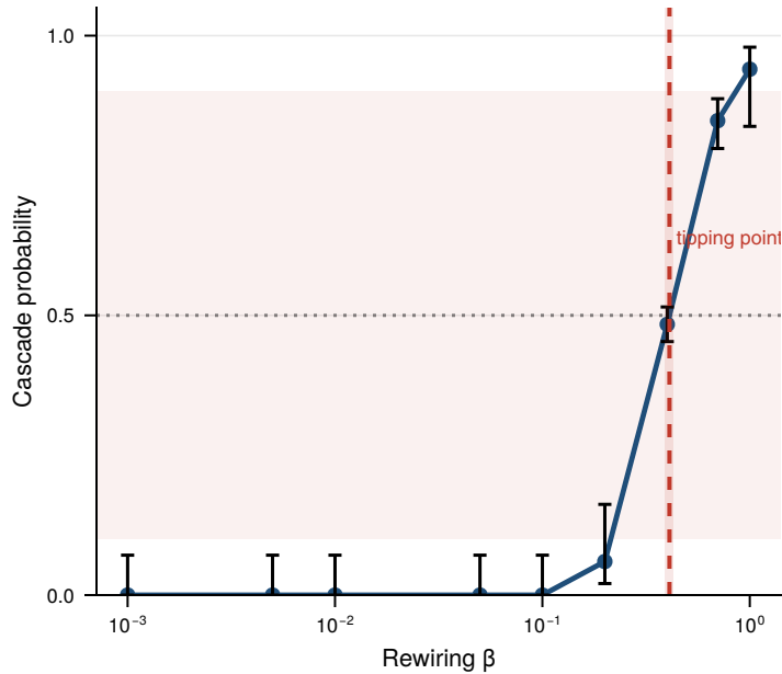
(a) Small-world: a sharp tipping point
