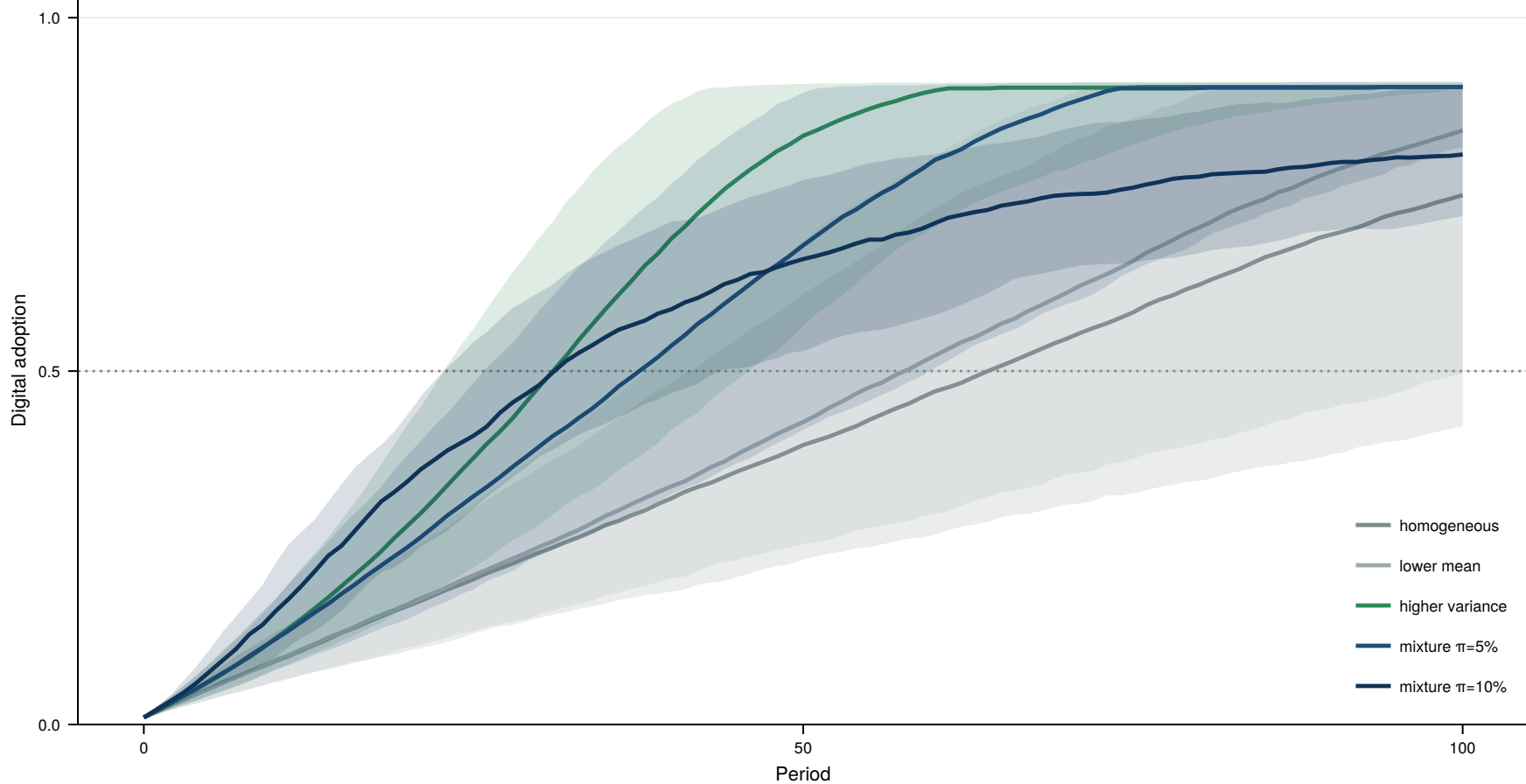
Adoption trajectories at \beta=0.4 , \theta=0.7 (median, 5–95% ribbon)
