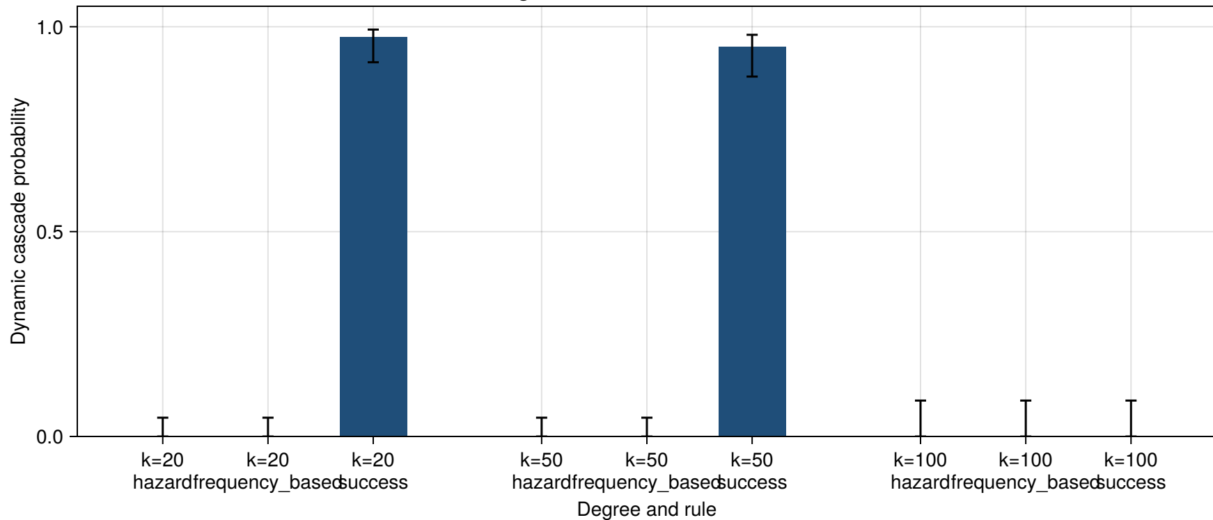
Realistic degree: success-conditioned rule vs nulls
