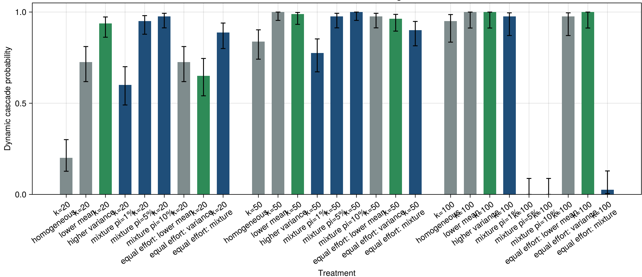
Threshold lower tails at realistic degree
