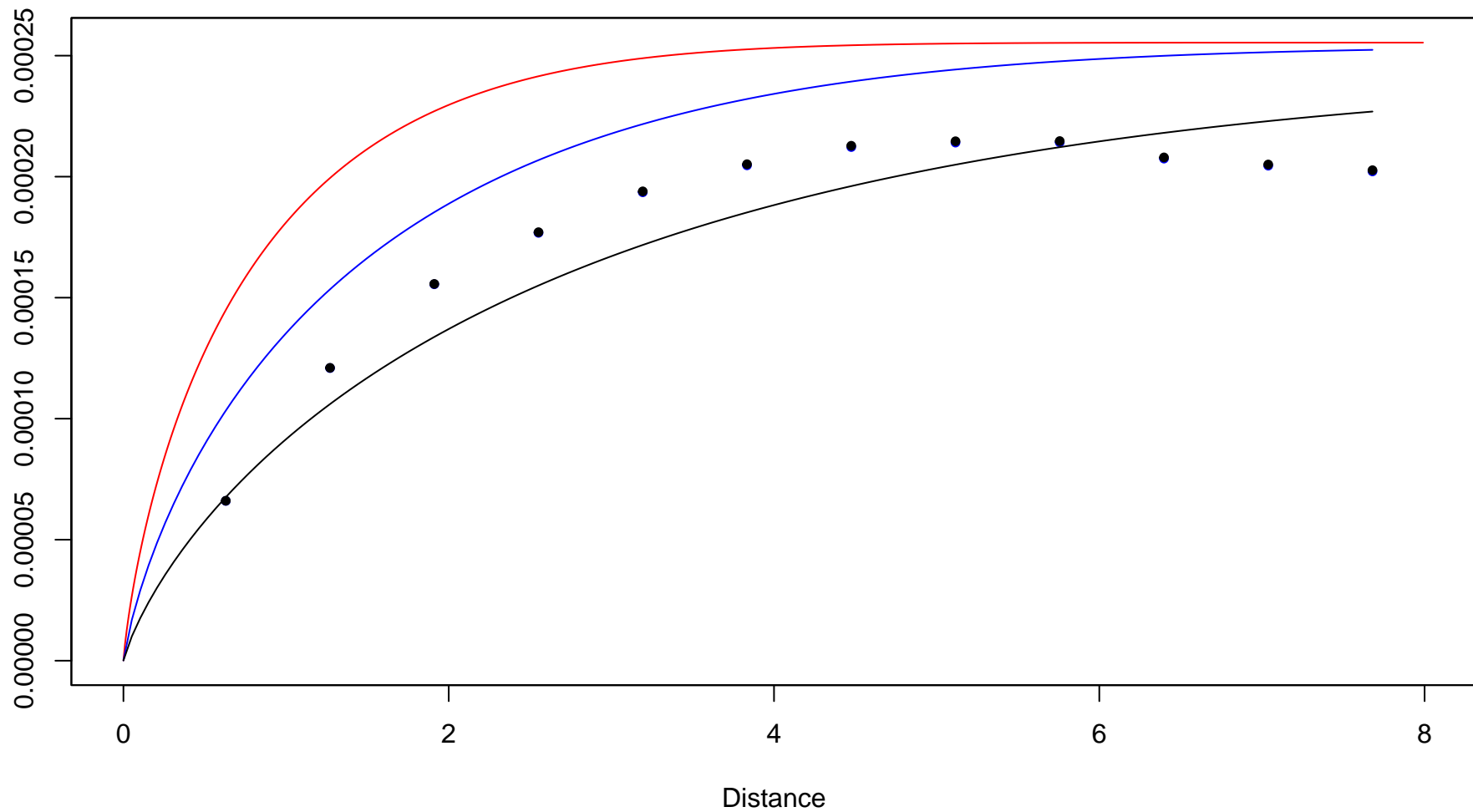
Semivariogram
