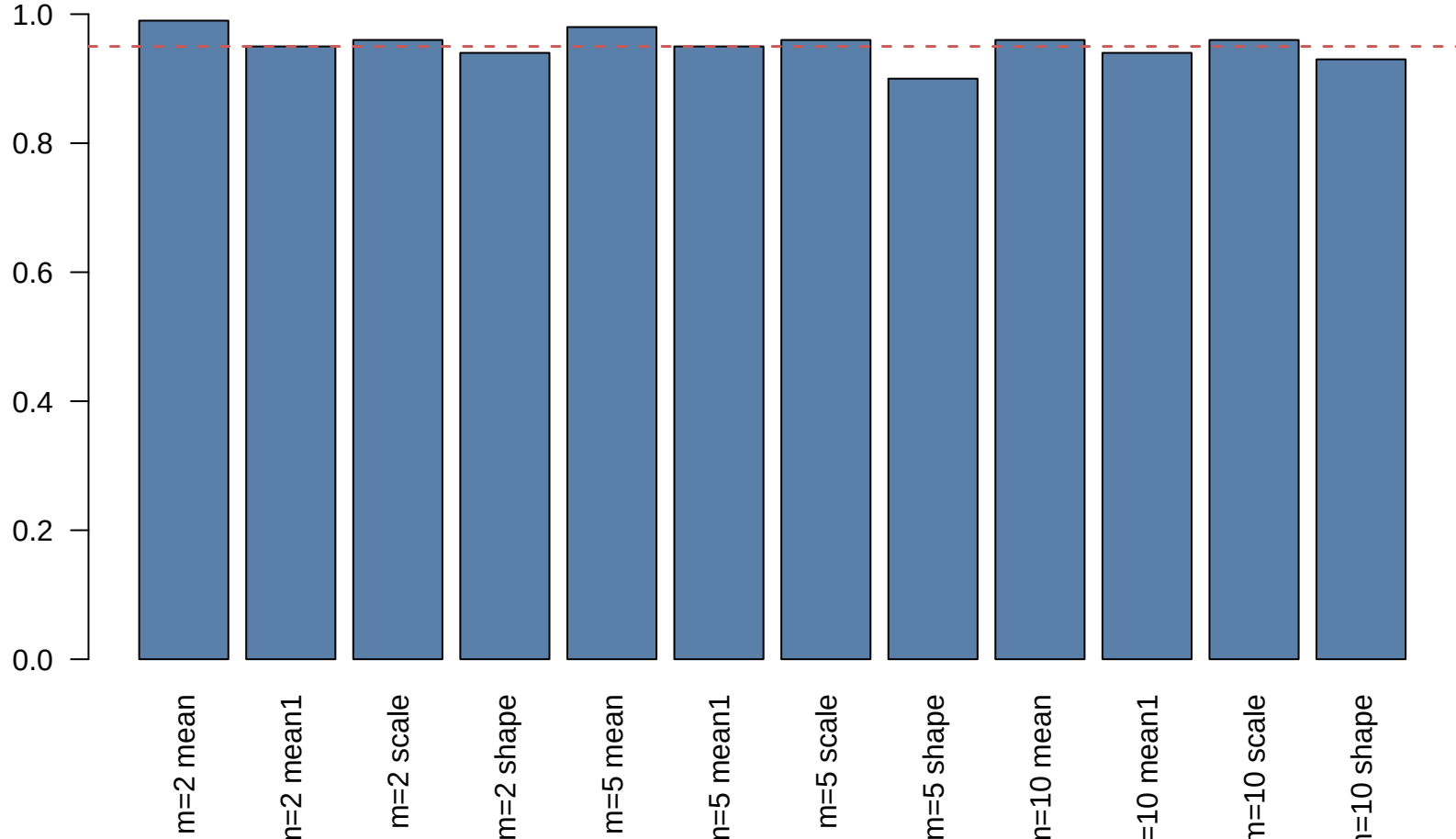
Empirical 95% coverage
