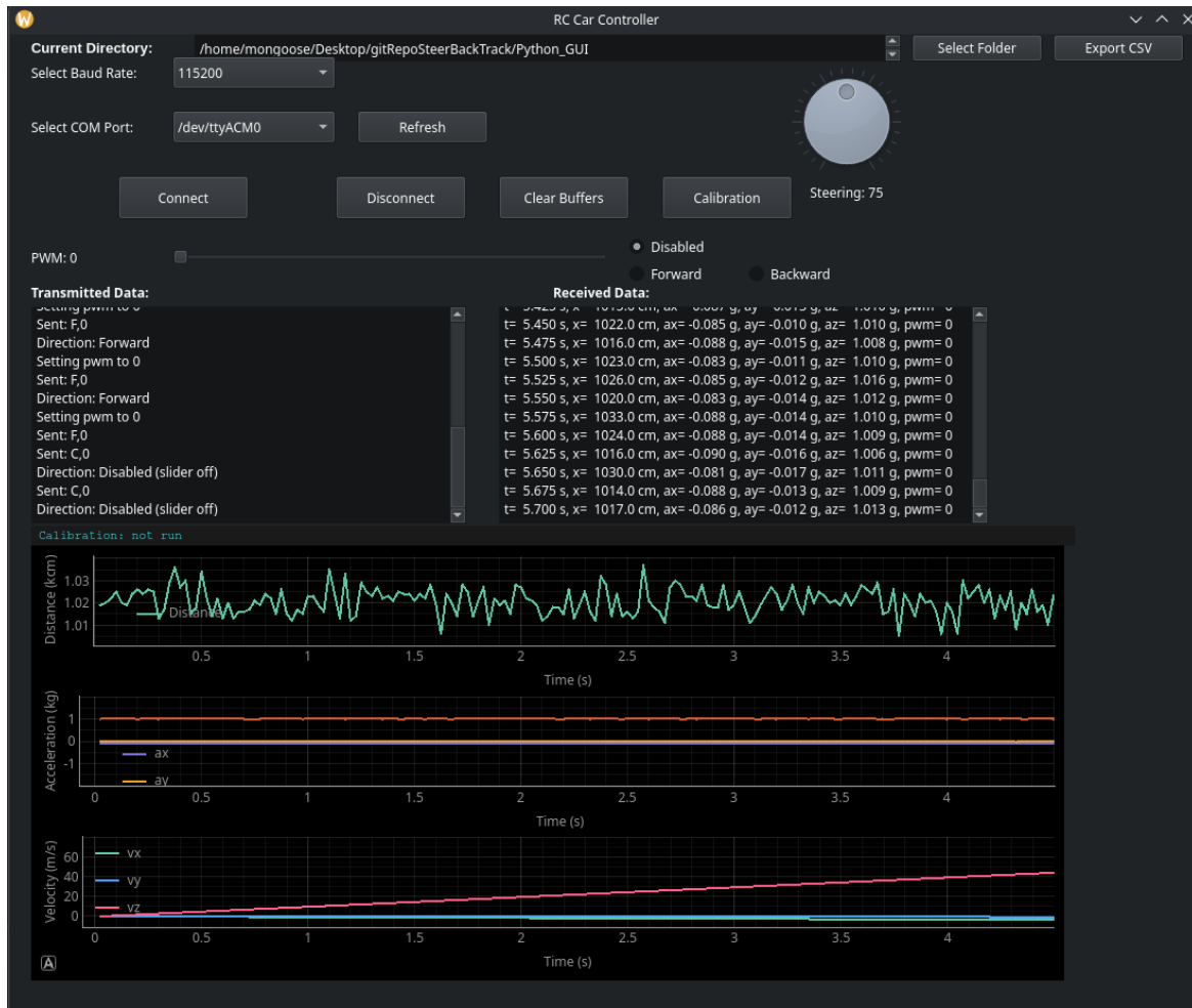
Fig. 18. The same User interface with no calibration.
