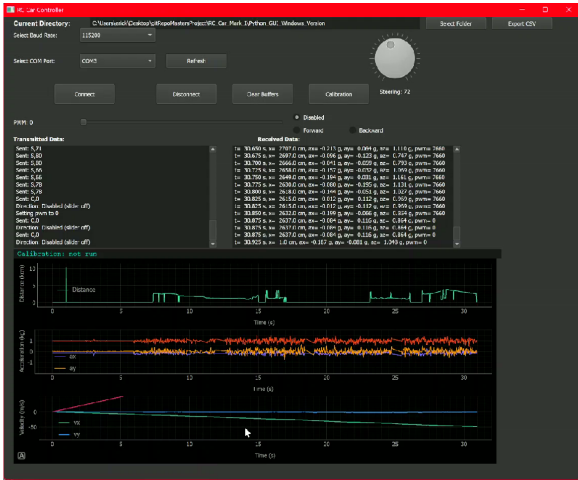
Fig. 17. The same User interface but with the x and y velocity component zoomed in.
