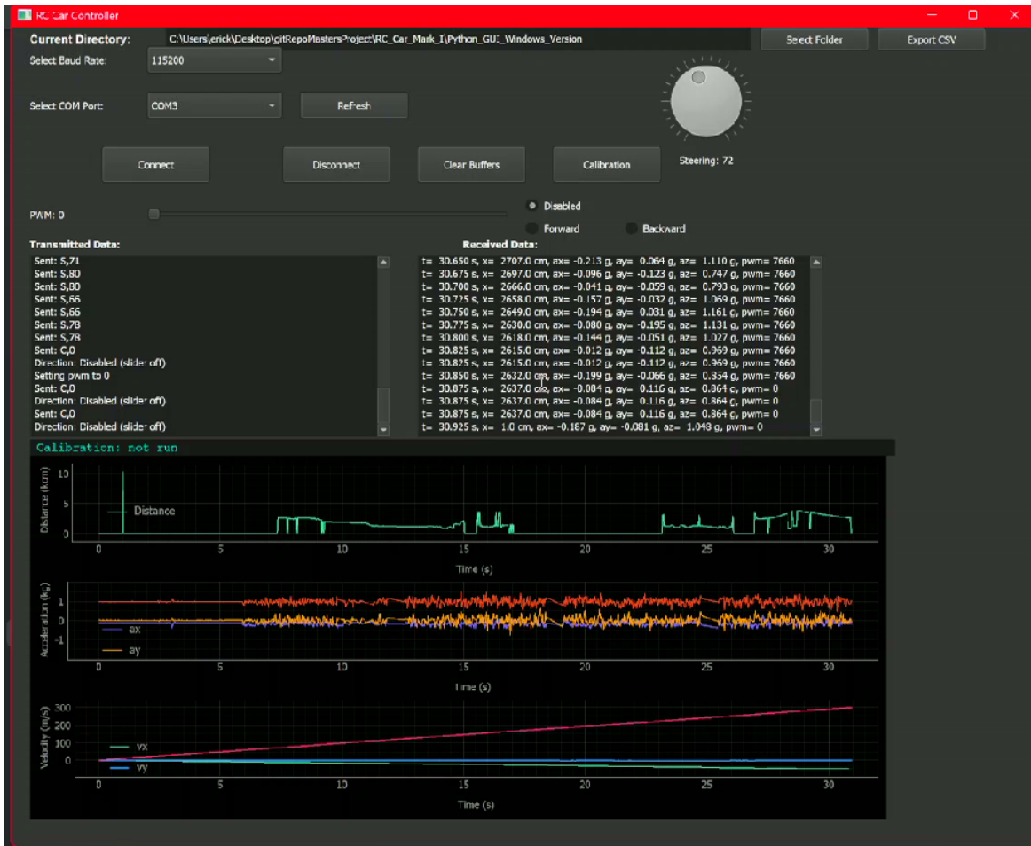
Fig. 16. The User Interface during the 30s test.
