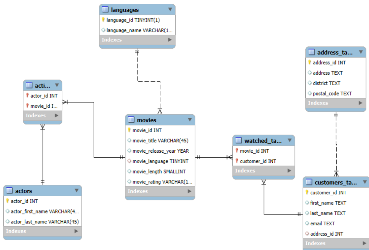
Figure 1 Movies ER Diagram (adaptation from sakila sample DB)
