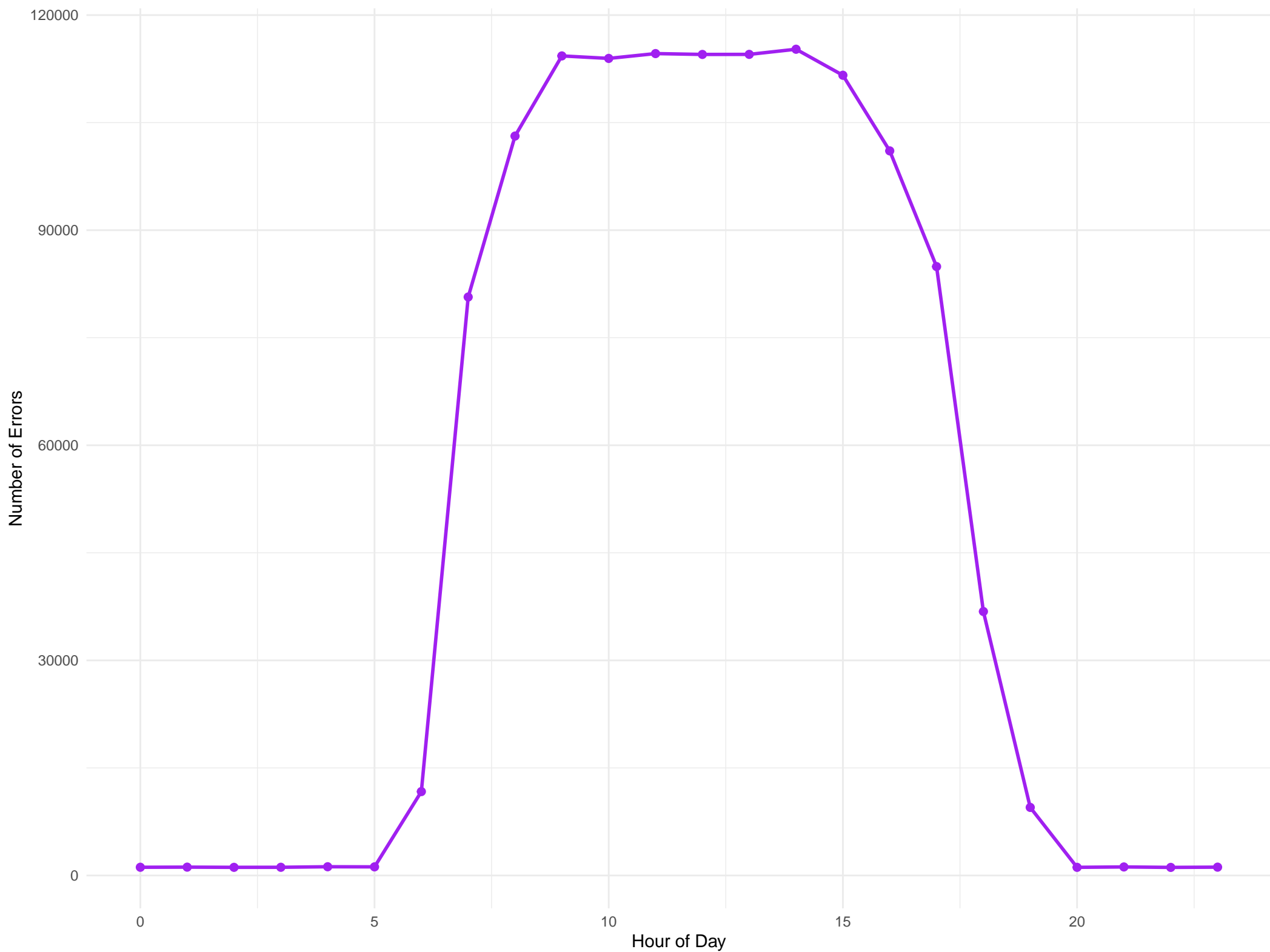
Hourly Pattern of Errors
