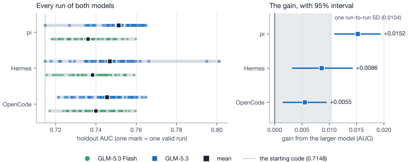
Figure 3. Left: every compliant run of both models, three agents. Black marks are the averages; the dotted line is the starting code. Right: the gain from the larger model with its 95 percent interval, against a shaded band one run-to-run SD wide.
