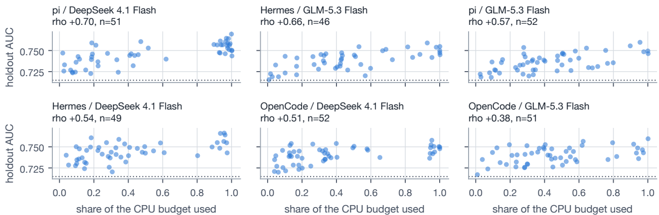
Figure 2. Budget use against score inside each pairing, compliant runs only. Dotted line: the starting code.
