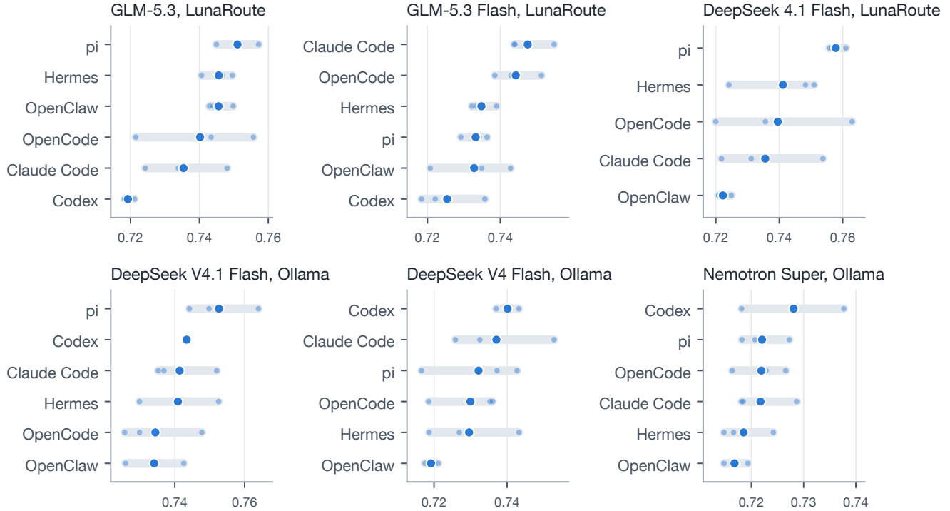
Figure 4. Holdout AUC, one panel per model row of Study 1. Per agent: the mean of three runs (large dot), the runs (small dots) and their range (bar).
