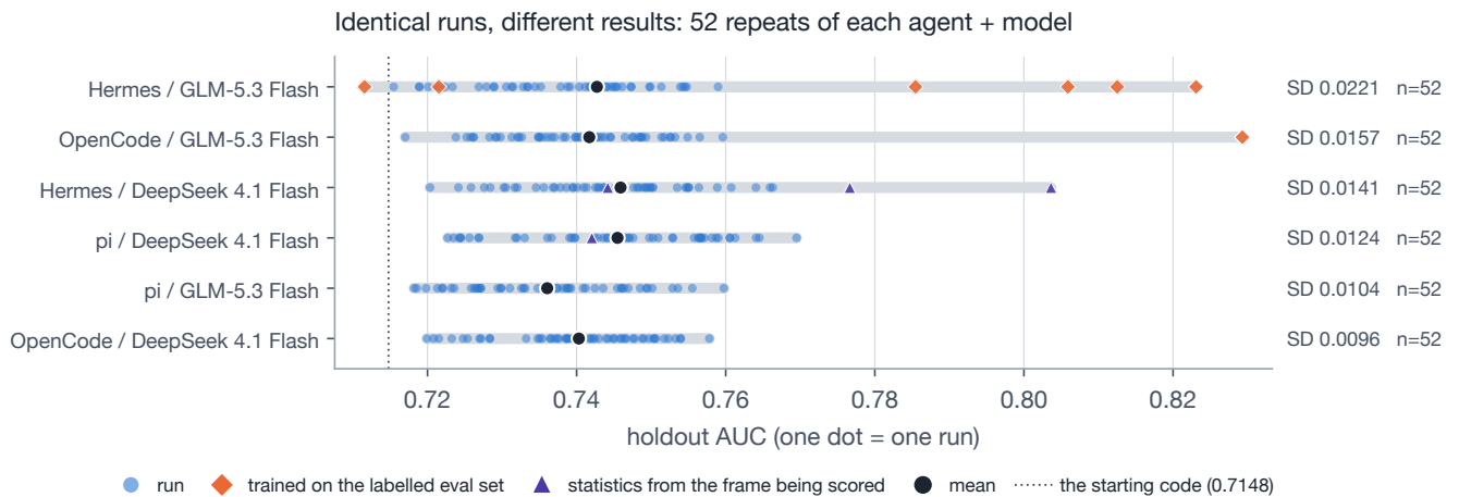
Figure 1. One dot per run, one row per pairing, sorted by variation. Black dot: the average. Dotted line: the starting code. Orange diamonds and violet triangles mark runs that broke a task rule.
