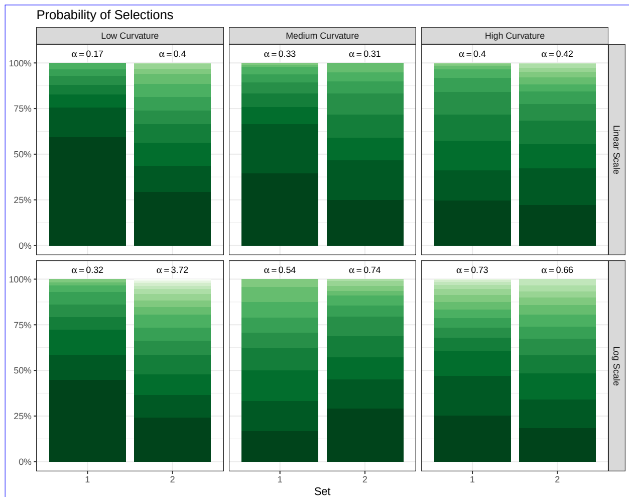
Figure 7: Observed proportions probabilities of panel selections for the 'Rorschach' lineups. The darker shade (bottom) denotes panels chosen more frequently than others. The annotated text provides the calculated \alpha parameter of the Dirichlet distribution that represents individuals' selections for the Rorschach plots.
