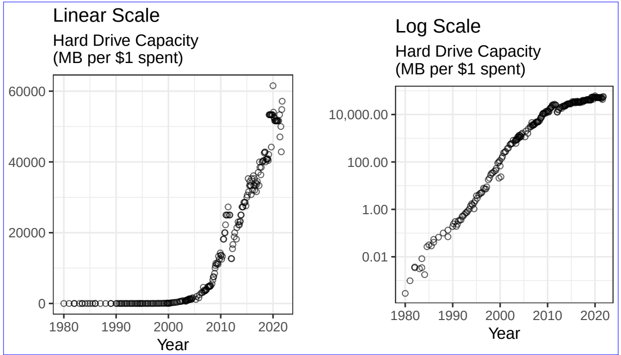
Figure 1: These plots present hard drive capacity ( mem, 2021 ) over the past forty years on both the linear and log scale and illustrate the use of the log scale when displaying data which spans several magnitudes.
