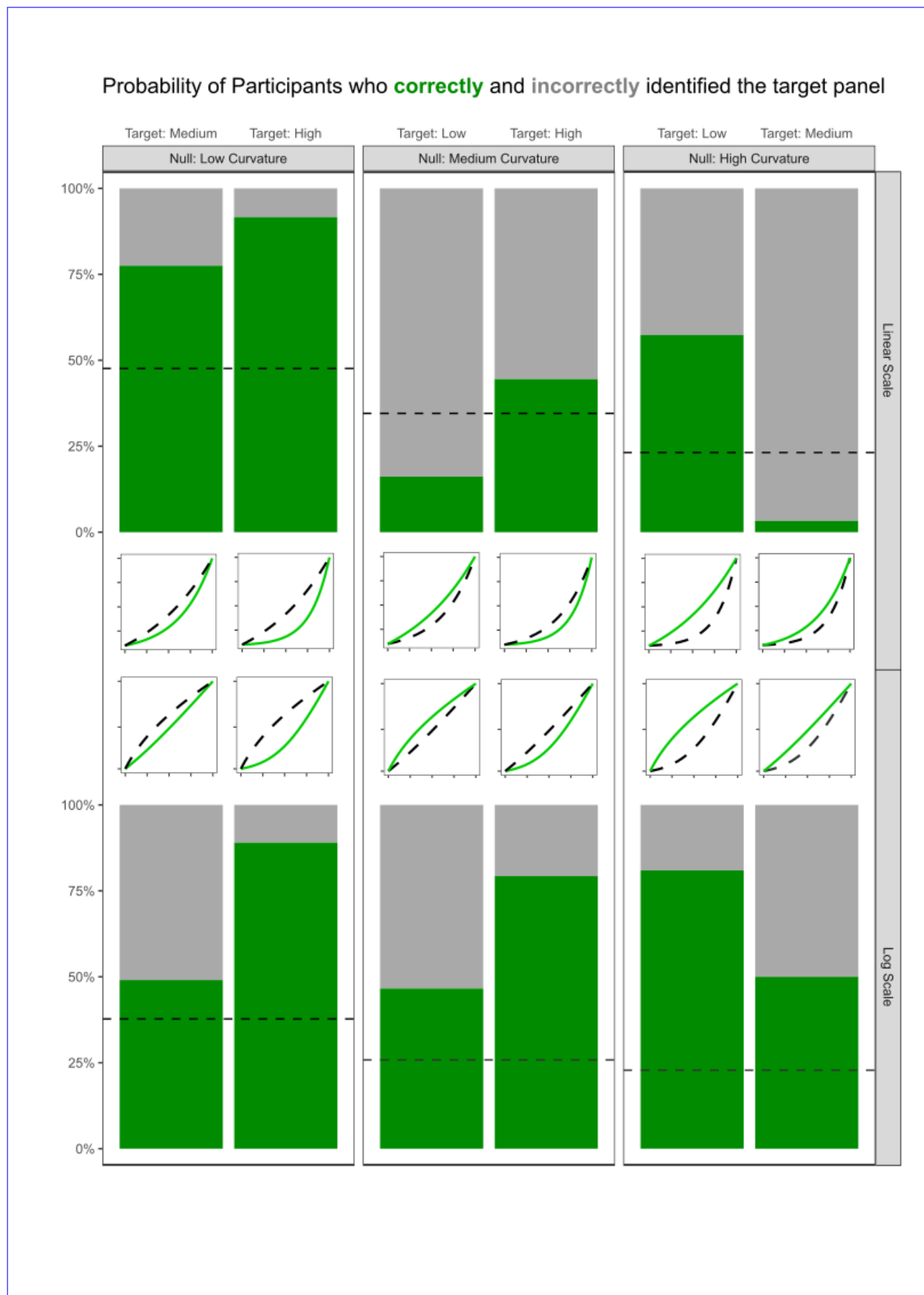
Figure 8: The observed accuracy for identifying the target panel for each curvature combi- 25
