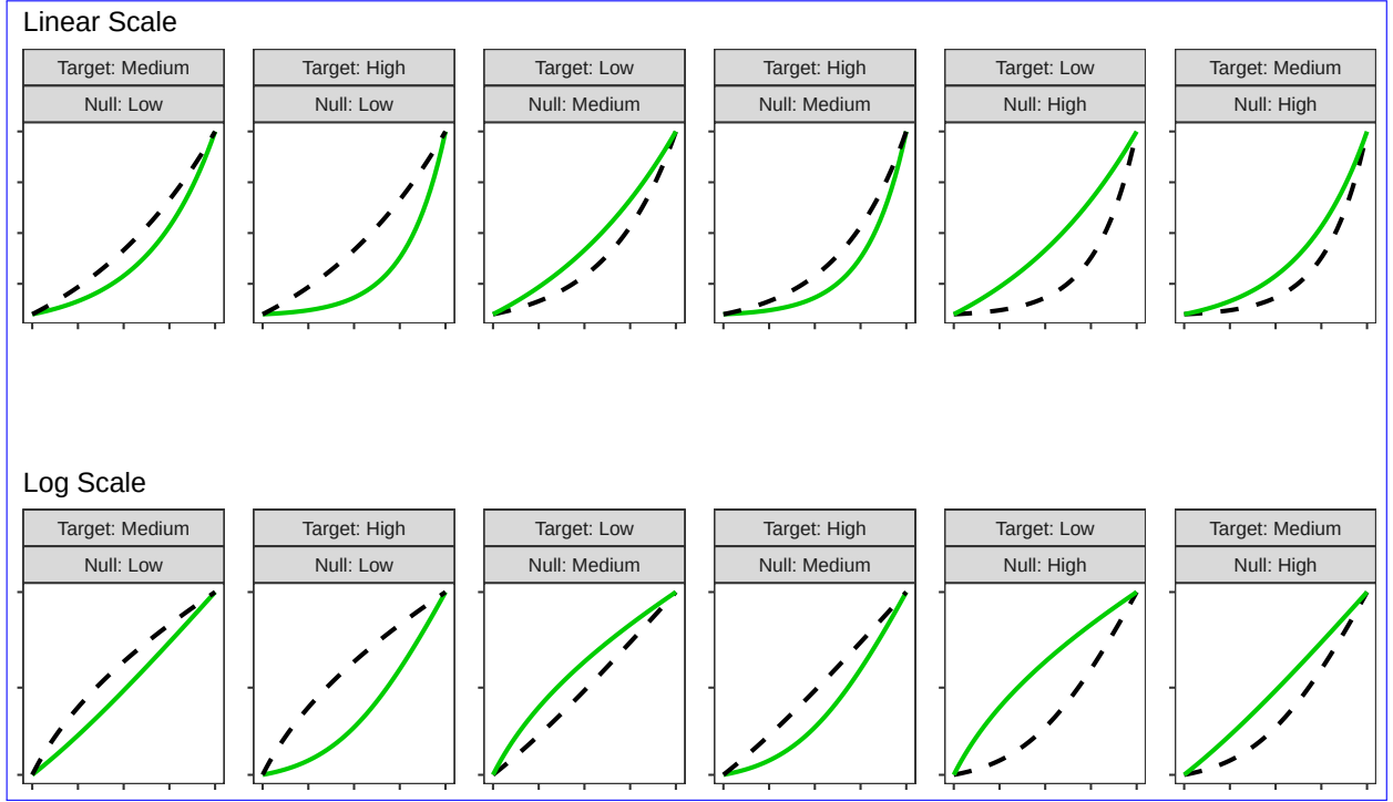
Figure 3: Thumbnail plots illustrating the six curvature combinations displayed on both scales (linear and log). The solid line indicates the curvature level to be identified as the target plot from amongst a set of null plots with the curvature level indicated by the dashed line.
