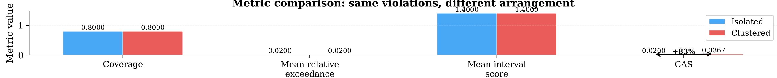
Metric comparison: same violations, different arrangement
