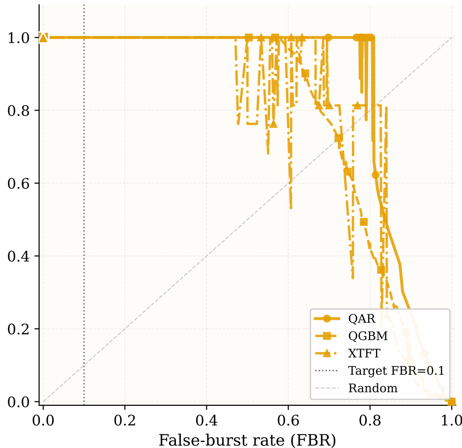
Operational risk-index: burst recall vs. false-burst rate (causal window h = 5 , \lambda = 1.0 , \gamma = 1.0 ; episode \geq 3 consecutive violations; detection within first 2 steps of onset)
