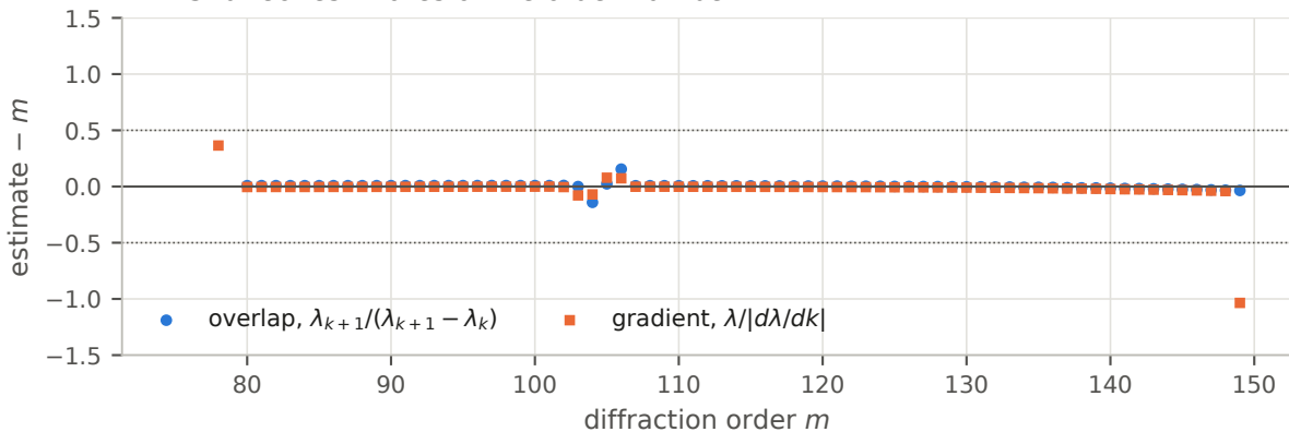
NIRPS: direct estimates of the order number
