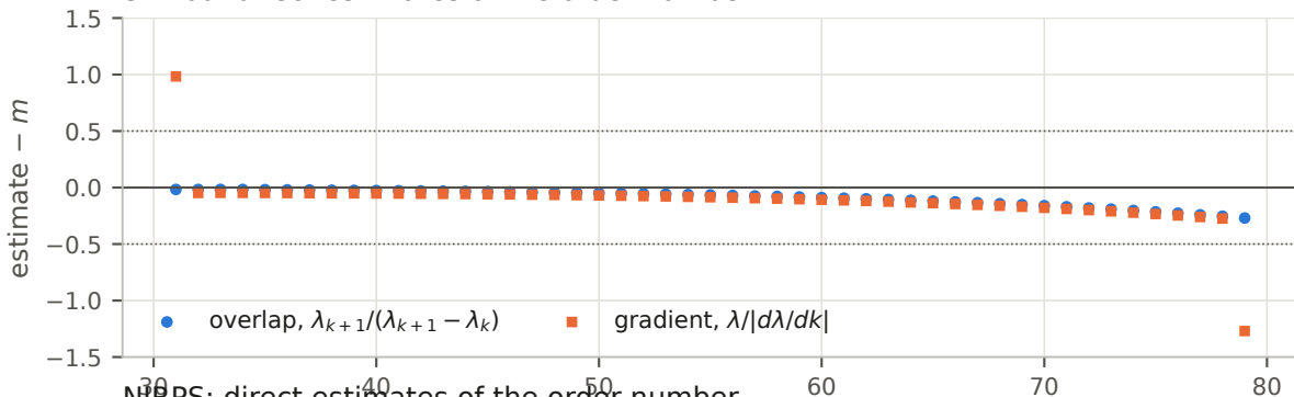
NIRPS: direct estimates of the order number
