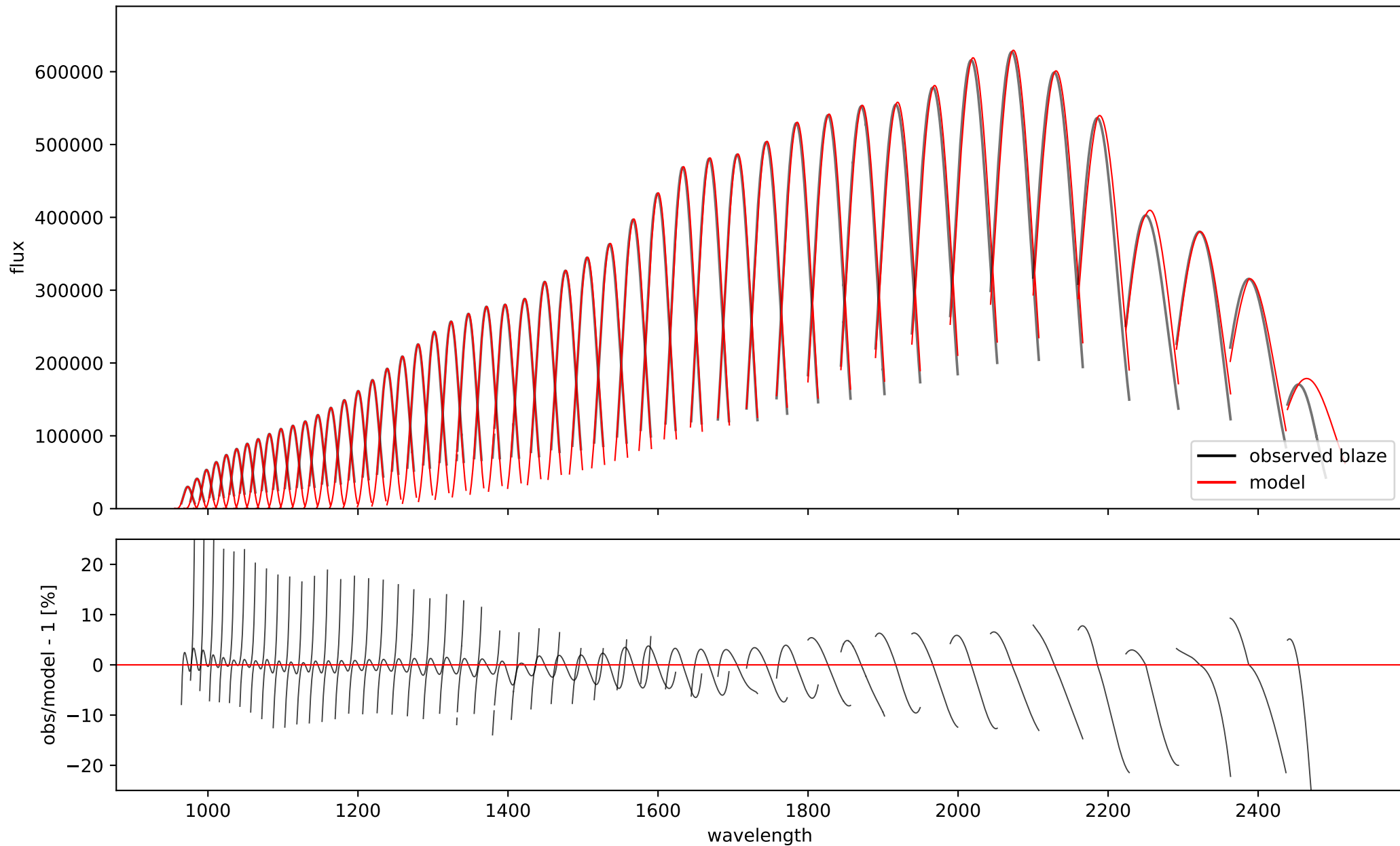
5000 K blackbody \times transmission (degree 1 spline) \times sinc 2 blaze \times d \lambda /dpix
